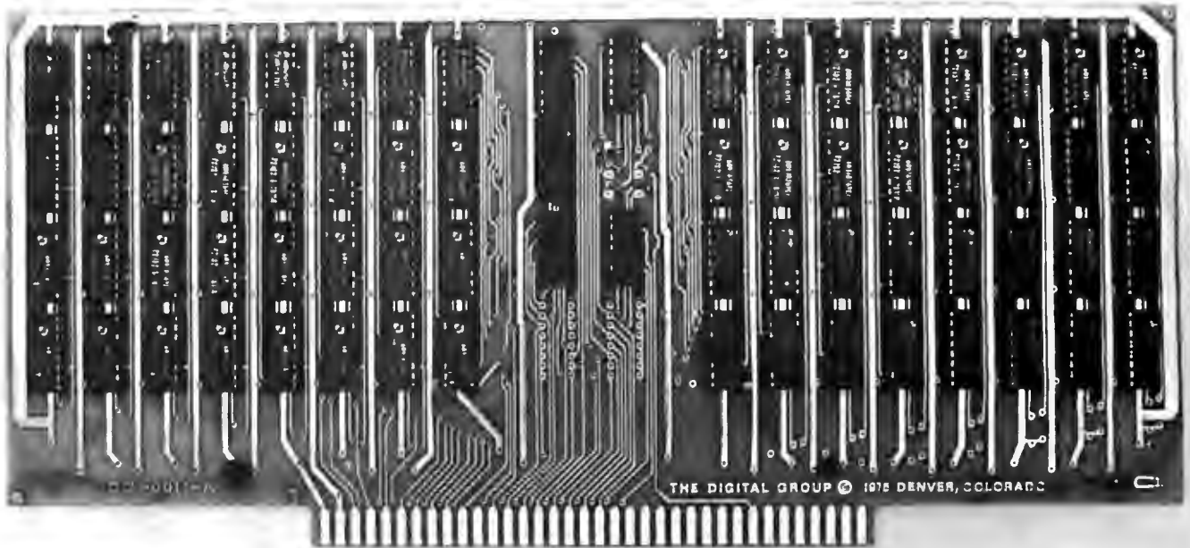
Photo 3: The author's Digital Group System 8 K byte memory card. The card contains 64 memory integrated circuits (in two arrayed segments) and in the center are various miscellaneous circuits used to interface the backplane bus of Digital Group system.
