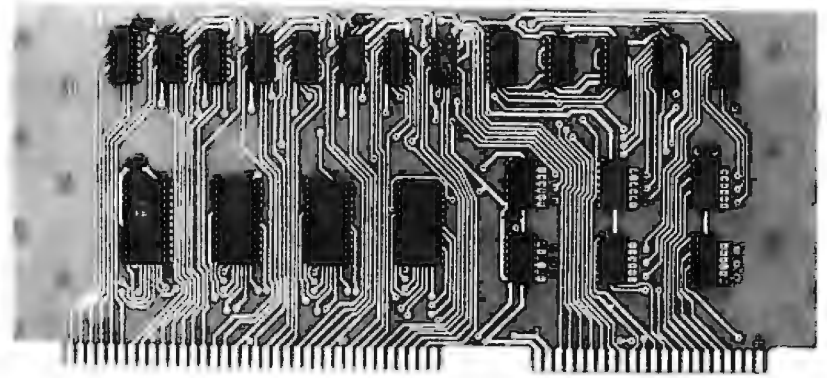
Photo 4: The author's Digital Group System IO card. This card interfaces to the system's bus, providing four parallel output ports and four input ports. These ports are routed to the backplane where they communicate to the video display, keyboard and cassette interfaces.
