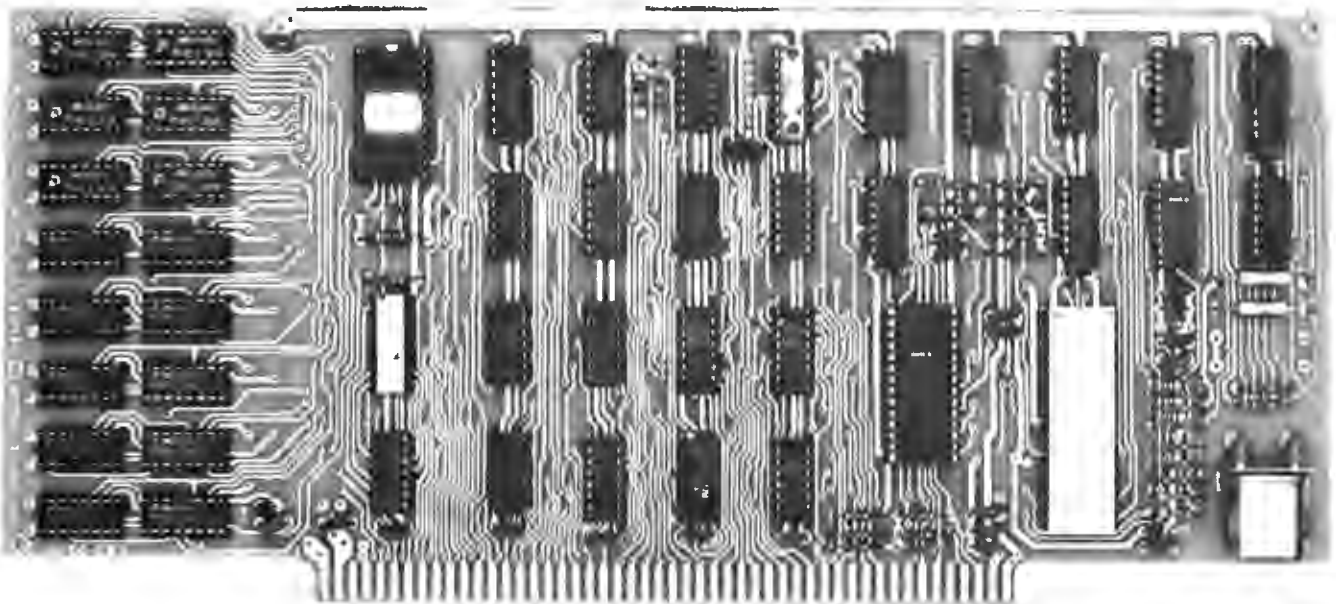
Photo 2: The author's Digital Group 8080 processor card. The actual processor is an AMD 9080A, one of the second sources of the original Intel 8080 design. The crystal which controls the processor clock is at the lower right, and the 2 K byte section of memory on the card is represented by the two rows of eight sockets at the left edge of the card. A UV erasable ROM chip (marked "80A" with a felt tip pen on the top edge at left of center) contains systems software which eliminates the need for a formal "blinkin' lights" front panel.
