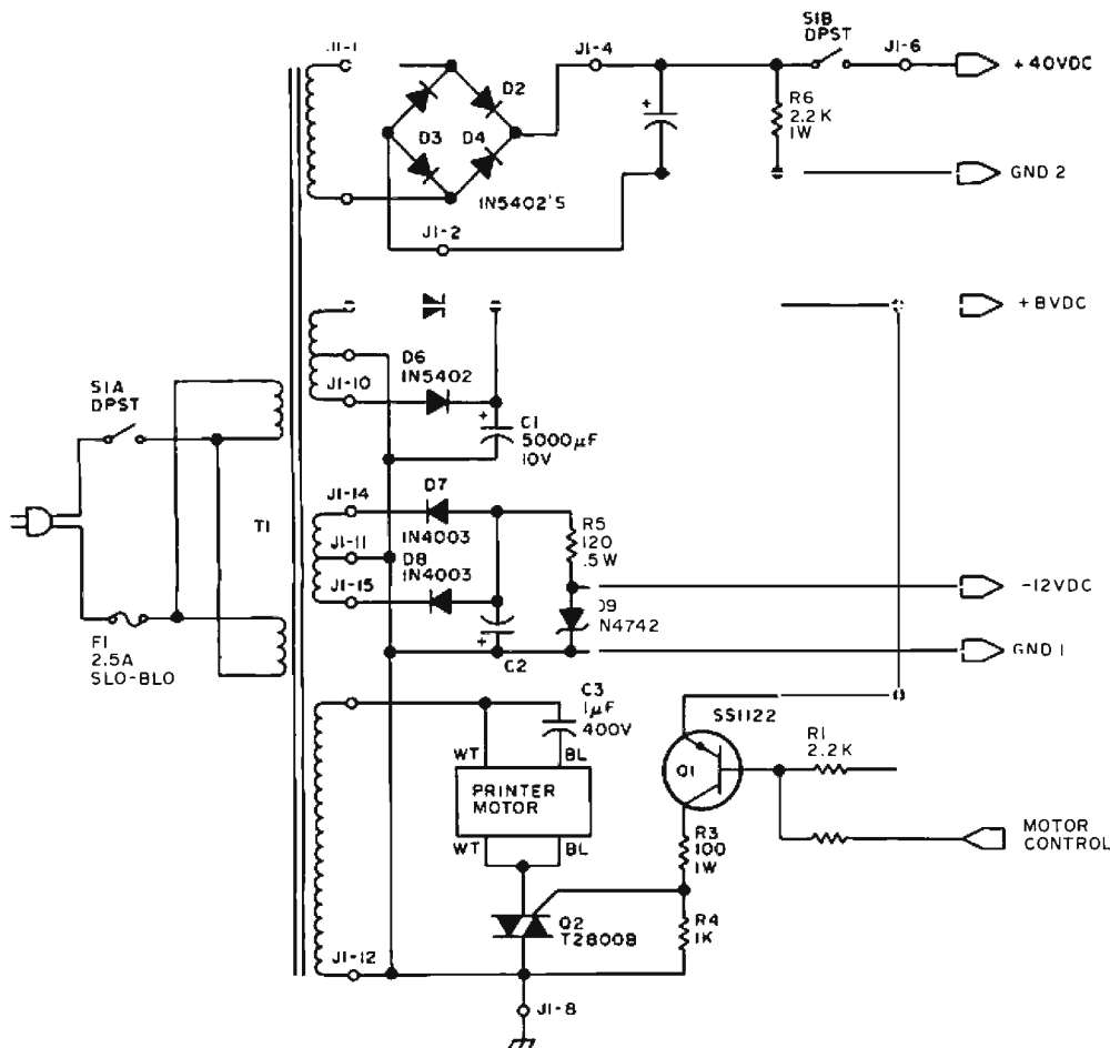
Figure 2: The schematic diagram of the power supply circuit for the PR-40 printer. This power supply can be run on either 120 or 240 VAC depending on whether the primary winding is wired in parallel or series. The power transformer, T1, has a 120, or 240 V primary; 32 V @2 A, 12.5 V @1 A center tapped, 120 V @200 mA center tapped secondaries. As can be seen in the diagram, the printer motor is triac controlled, taking its on and off states from the position of the printer head on the page. All resistors are measured in ohms and are 0.25 W unless otherwise stated.
