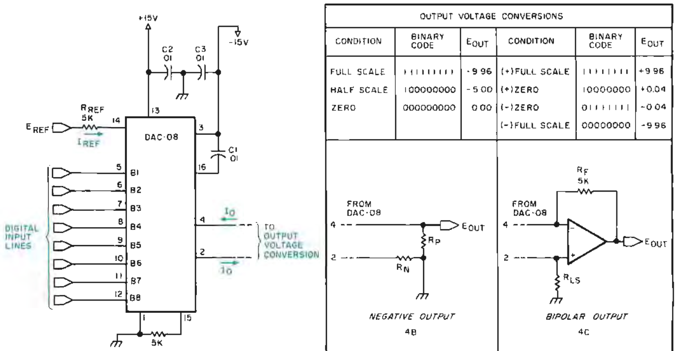
Figure 2: While the circuit of figure 1 could be constructed, it is usually more convenient to replace it with a monolithic integrated circuit device such as the DAC-08 part by Precision Monolithics, which is used for this illustration. The integrated circuit contains all the components of the R-2R network of switches and buffering amplifiers. It still requires an output conversion circuit (two variations shown) and a reference voltage. Because the R-2R network is an integrated circuit, this form guarantees the highest possible accuracy with none of the extra bother of hand wiring a circuit as in figure 1.
