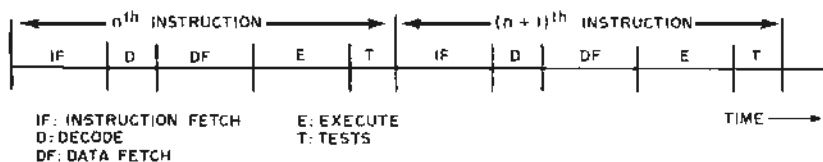
Figure 6: Timing diagram for the sequence of interpreting an instruction. This process is divided into five stages: instruction fetch, decode, data fetch, execution and testing. As soon as the testing is finished, the instruction fetch cycle is again encountered to start the next sequence.
