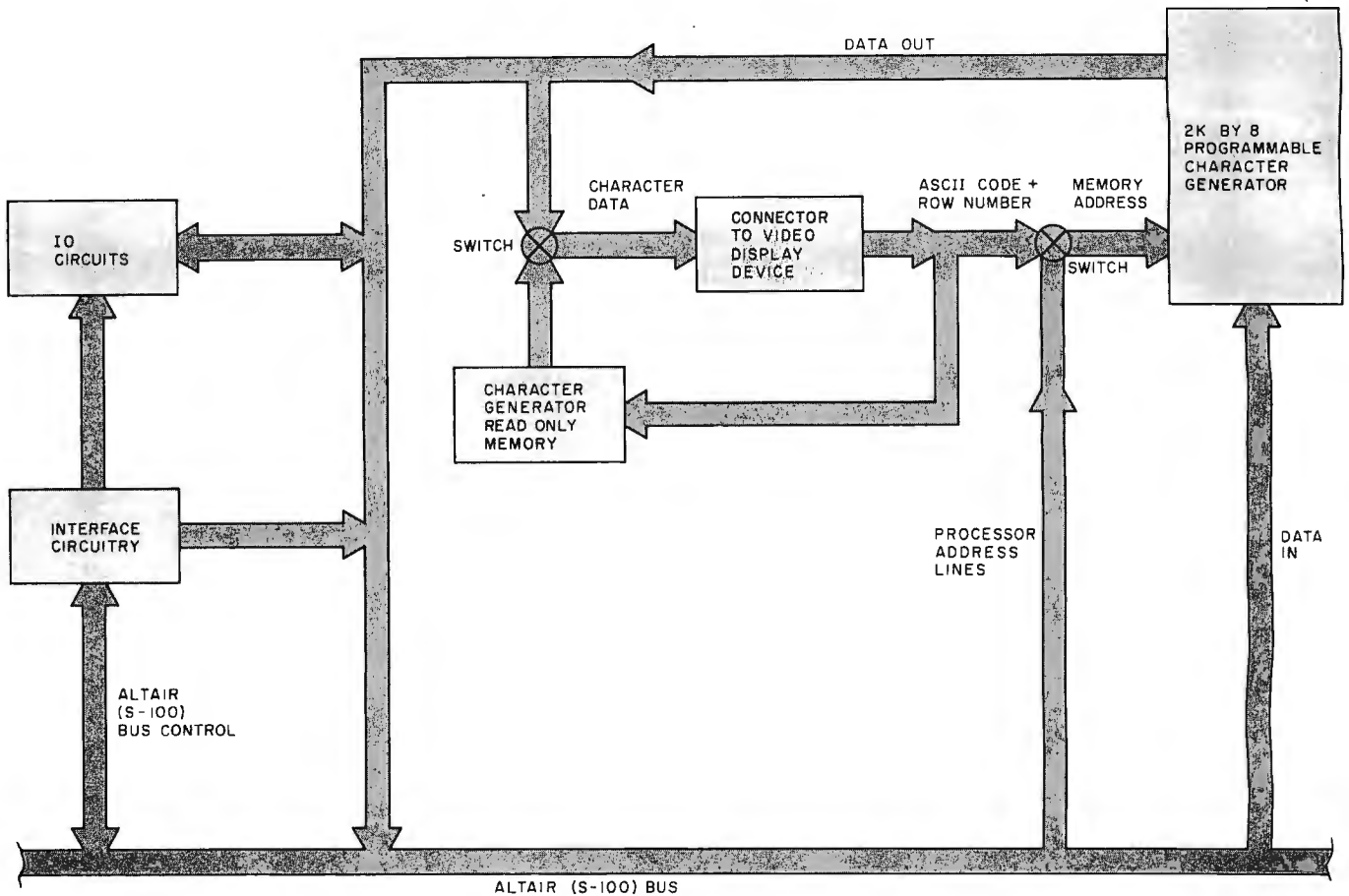
Figure 2: Detailed block diagram of the programmable character generator circuit. The circuit consists of 2 K bytes of programmable memory containing custom characters. This memory is addressed by the character and row lines that normally go to the existing character generator on the video display board. These lines are multiplexed with the normal processor address bus lines. Hardware and software switches determine whether data from the existing character generator or data from the programmable character generator will be used to feed the video display.
