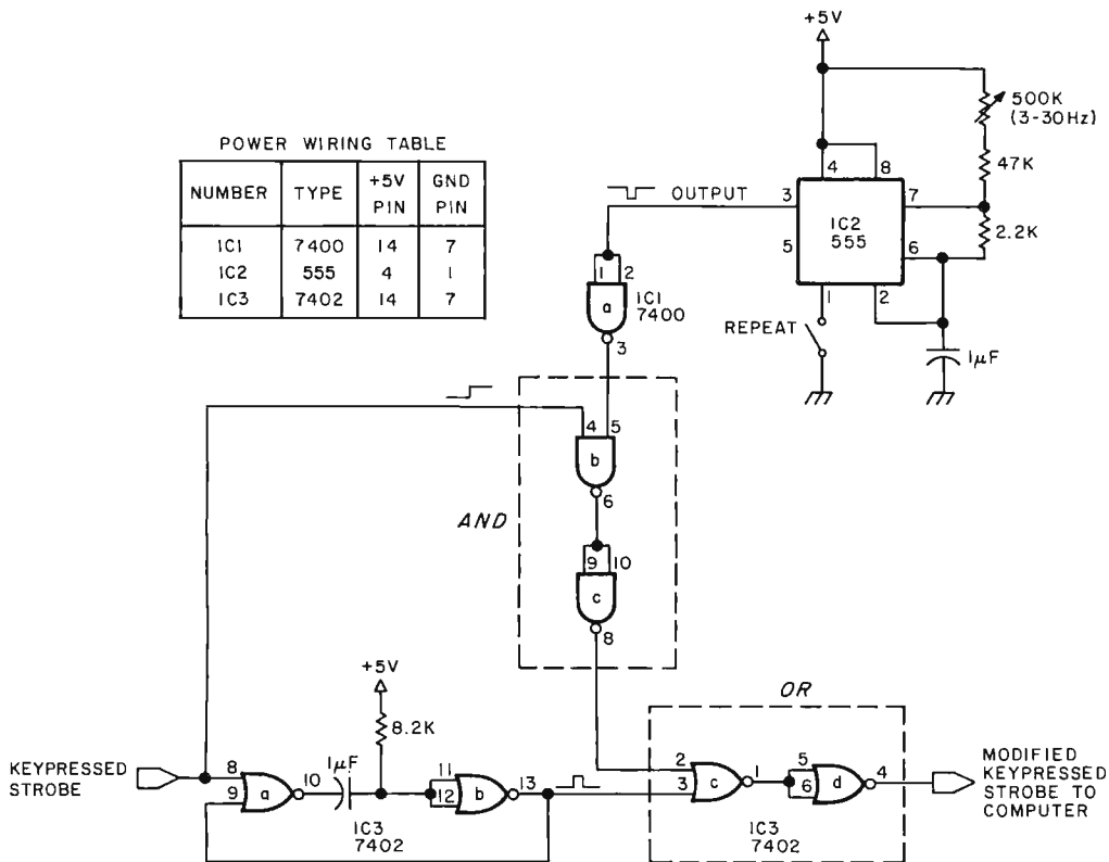
Figure 1: Interface circuitry for GRAPH. An astable multivibrator (IC2) provides the pulse train for a hardware repeat function. The authors' keyboard produces a low to high transition strobe (STB) pulse when a key is pressed. This is used to trigger a monostable multivibrator to provide a single pulse keypressed (KP) signal to interface with the IO board used.
