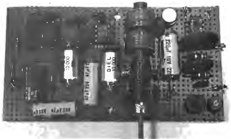
Photo 2: Internal view of finished prototype receiver chassis.
