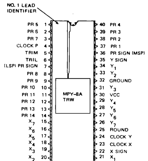
Figure 1: Physical layout and pinout diagram for the MPY-8AJ multiplier part, reproduced from the specifications sheets, courtesy of TRW Electronic Systems Division, One Space Park, Redondo Beach CA 90278. Note that bits are numbered from 1 (most significant) to n (least significant), a convention which differs from conventional microprocessor usage in which bit 0 is always the least significant. The text and figures of these articles reflect the inverse ordering of the bit numbers on the multiplier side of the interface.
