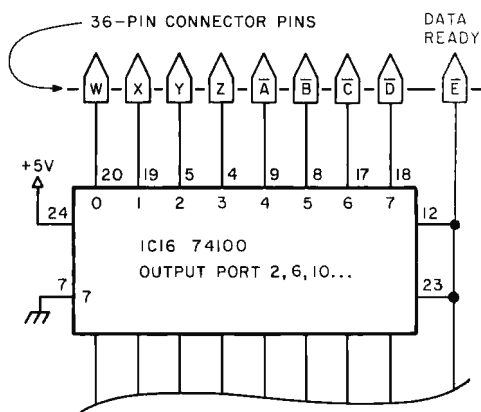
Figure 3: Modification to the Digital Group IO board. The Z-80 processor, which forms the heart of the Digital Group computer, features a block output instruction (OTIR) that can output 1 byte every 9 \mu s using the standard 2.5 MHz clock. This degree of speed is needed to output the data needed for the 3-D display without using direct memory access circuitry. Adding the data ready line (shown in grey) to IC16 (Digital Group numbering) creates a status signal to the mirror circuitry. This avoids the necessity of using output bits from another port for this purpose, which would slow down the data transfer rate. (The choice of port 2 for the output port is particular to the authors' system.)
