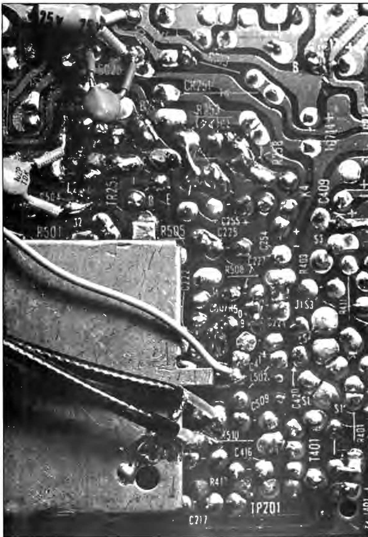
Photo 5: This view shows where modifications must be made to the underside of the Hitachi SX chassis printed circuit board. A foil trace carrying the video signal is cut and routed through shielded wire to the external switch, and a small disk capacitor (at top with spaghetti tubing on legs) is attached across a spark gap to improve the set's response to abrupt black and white changes.
