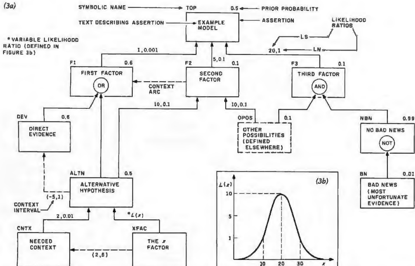
Figure 3: Diagram showing some of the constructs used in the PROSPECTOR inference networks. In figure 3a, boxes represent assertions. Each assertion's symbolic name is at the upper-left corner of the box and text describing the assertion is inside the box. Most assertions have prior probability values shown at the upper-right corner of the box. Evidence can be combined by logical connectives such as AND, OR, and NOT, represented by circles inside boxes; by plausible inference rules, indicated by two rule-strength values, LS and LN (LS indicates how sufficient the evidence is for establishing the hypothesis, if the evidence is present; LN indicates how necessary the evidence is for the hypothesis), and by variable likelihood ratios L(x) , defined in figure 3b. Dashed arrows indicate contextual constraints, which can "turn on or off" one question or a whole section of the network (at the tail of the arrow), depending on the answer to another question (at the head of the arrow). Figure 3b shows a plot defining a likelihood ratio L(x) for a numerical answer x to a question from PROSPECTOR. The likelihood ratio depends on the numerical value provided by the user.
