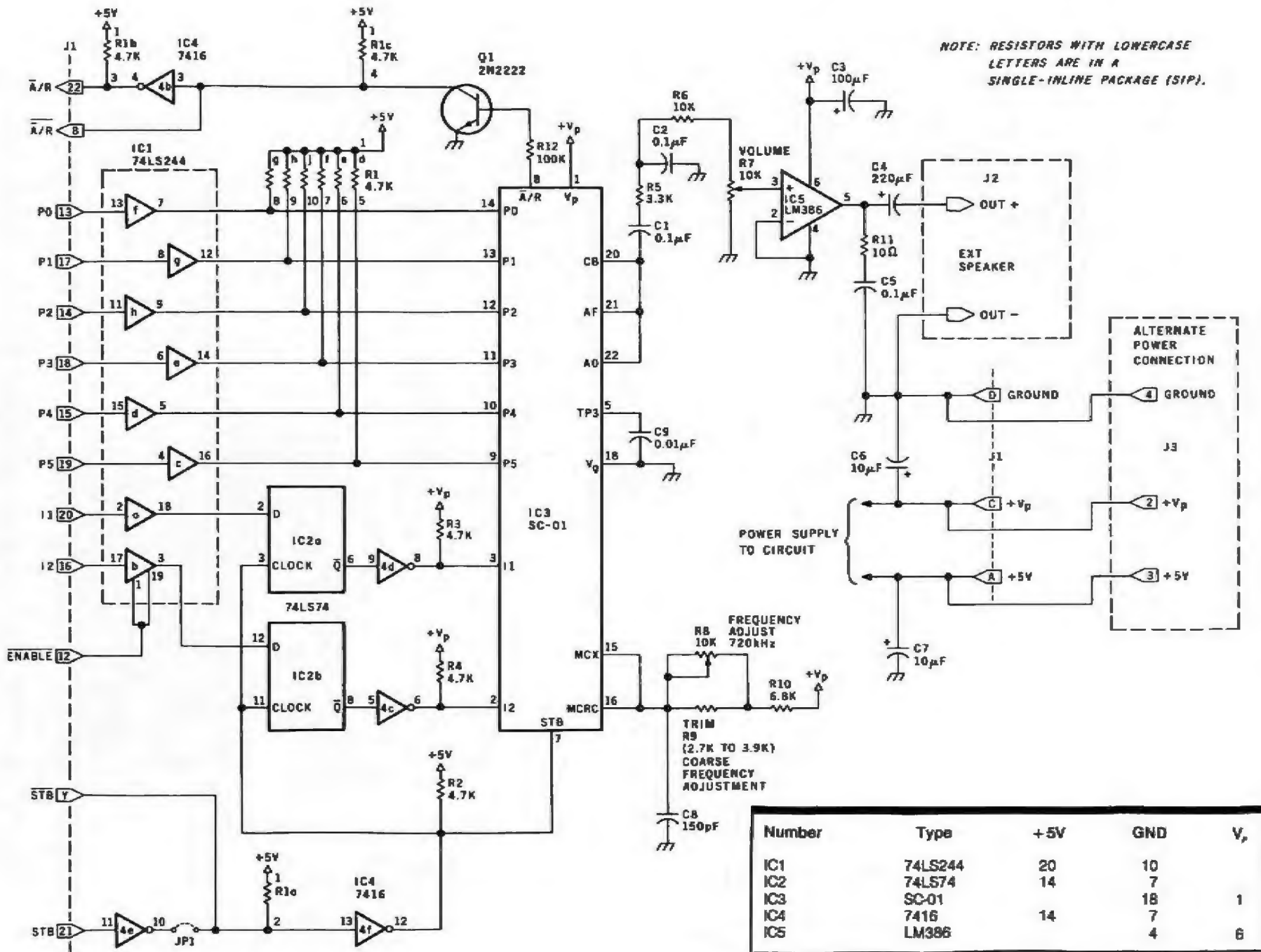
Figure 4: Schematic diagram of the Sweet Talker phonetic synthesizer in the parallel-port version.
