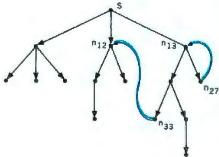
Figure 2: A directed graph. This figure, which represents the structure of many "real-world" problems, differs from a tree in that successors may be in the same or a "shallower" depth (note colored arrows). The successor of n_{33} is n_{12} ; the successor of n_{27} is n_{13} . Tree-searching algorithms can be modified to handle graphs, but this article will deal exclusively with trees.
