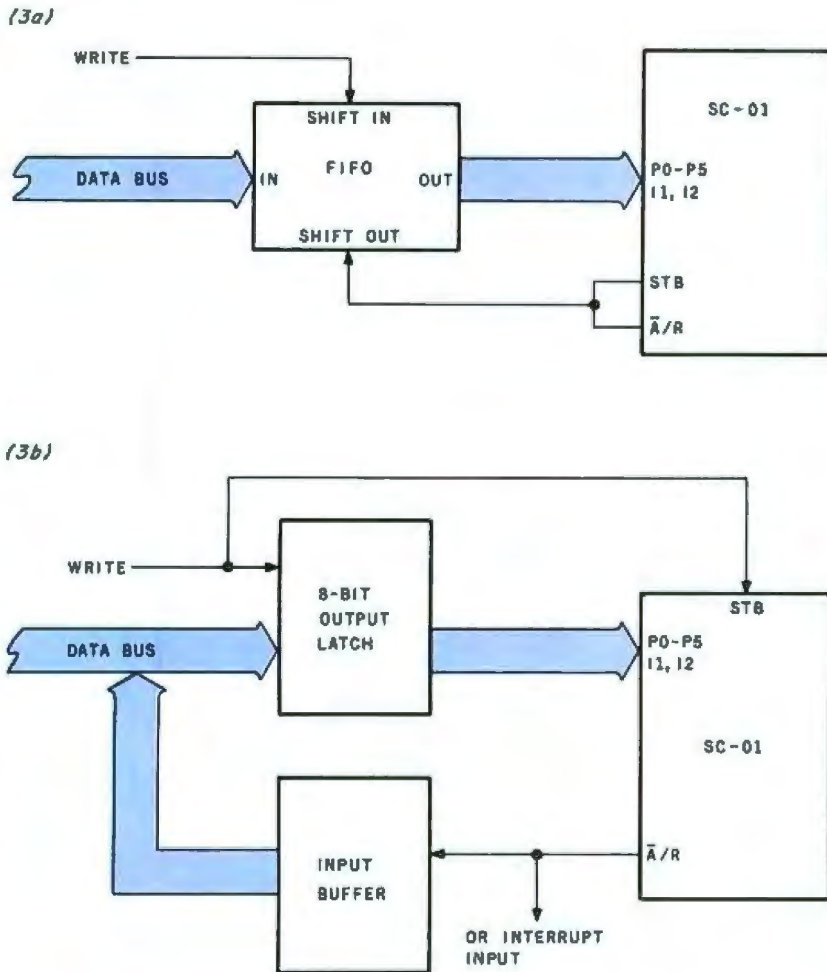
Figure 3: Two methods of interfacing the SC-01 to a microcomputer data bus. Figure 3a shows an independently acting, self-timed circuit with a FIFO (first-in, first-out) buffer. Figure 3b shows a circuit that allows the computer to time the transmission of data to the SC-01.
