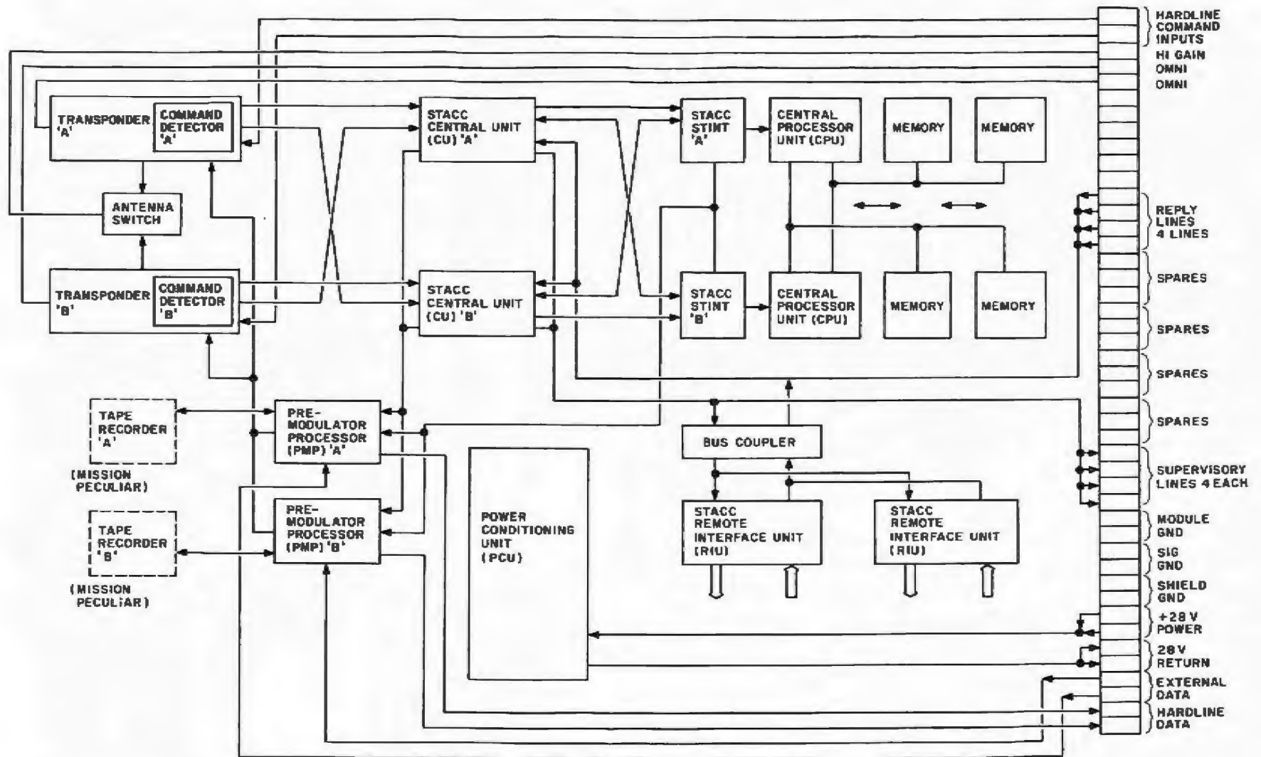
Figure 3: Detailed block diagram of the Command and Data Handling Module of the Multimission Modular Spacecraft. The diagram shows the module's interface as well as the redundancy of each of the module's components.
