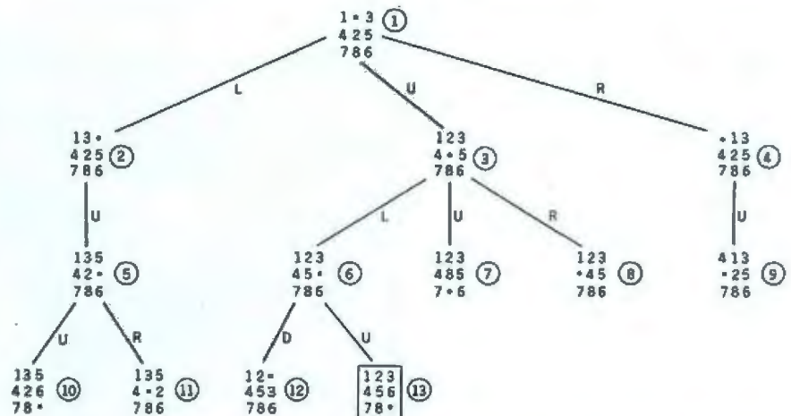
Figure 10: Solution to the puzzle (3, 2) by the breadth-first algorithm. The circled numbers to the right of each node indicate the order in which they are expanded. Nodes 8 through 13 (six nodes) are "open" (ie: they have not yet been expanded), whereas nodes 1 through 7 are "closed."
