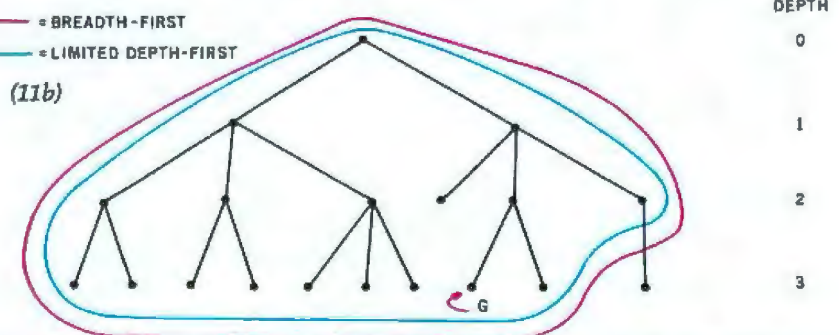
Figure 11: A comparison of search efficiency. The limited depth-first search always produces the same or fewer nodes than the breadth-first search, when the depth of the search is equal to the depth of the goal node. An example of the efficiency of the limited depth-first search is shown in figure 11a, where the breadth-first search (indicated in color) has produced more nodes. In figure 11b, the two types of searches produce an equal number of nodes, using the same partial tree but a different goal node. The breadth-first search must always expand the entire tree to depth n-1 , whereas the limited version may not, depending on the location of the goal node.
