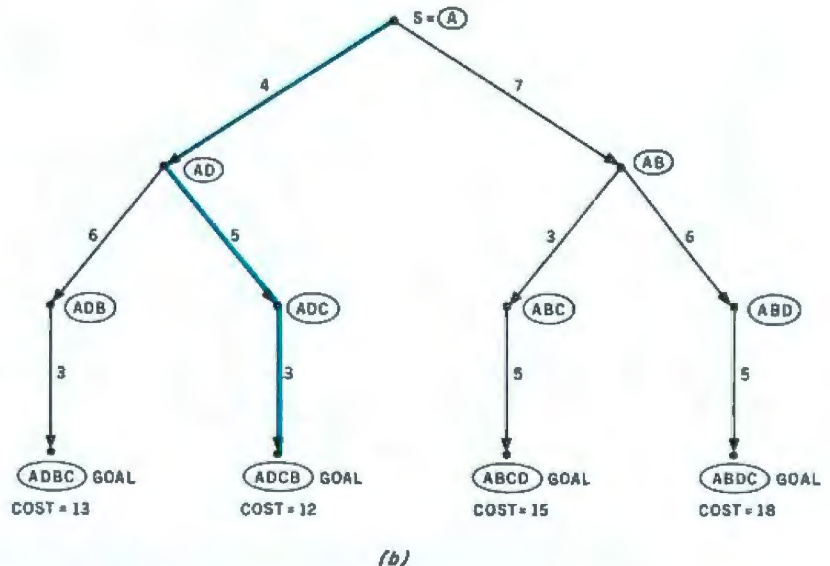
Figure 3: The traveling-salesman problem. Given the map in figure 3a, the objective is to find the shortest route from city A through cities B, C, and D. The tree of figure 3b gives the finite-state representation of the problem, with each node being a partial trip (eg: ADC is the trip from A through D and C) that has a cost dependent upon the route taken. Here the problem is discrete, and any node has only a finite number of successors; at node AD, only two "next moves" are possible: ADB and ADC. The shortest route is shown in color.
