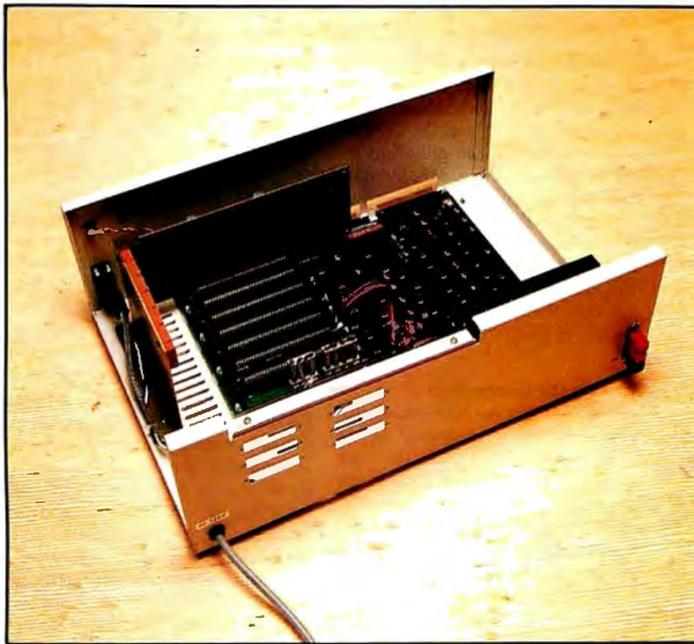
Photo 9: The NEC PC-8012A I/O unit has seven slots for expansion and connectors on the back that can carry nonstandard voltages to the bus.
