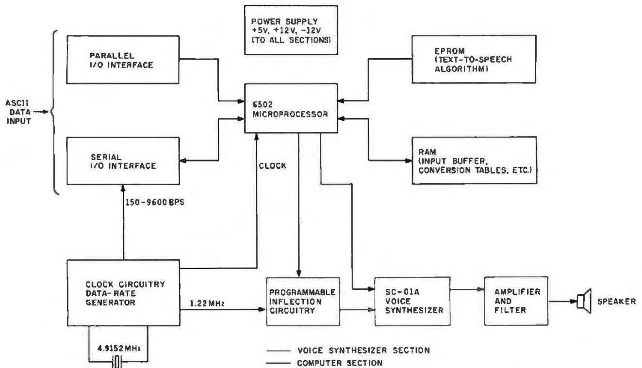
Figure 2: Block diagram of Microvox. The Microvox hardware can be viewed as a general-purpose 6502-based computer with a speech synthesizer attached using a memory-mapped I/O (input/output) port.
