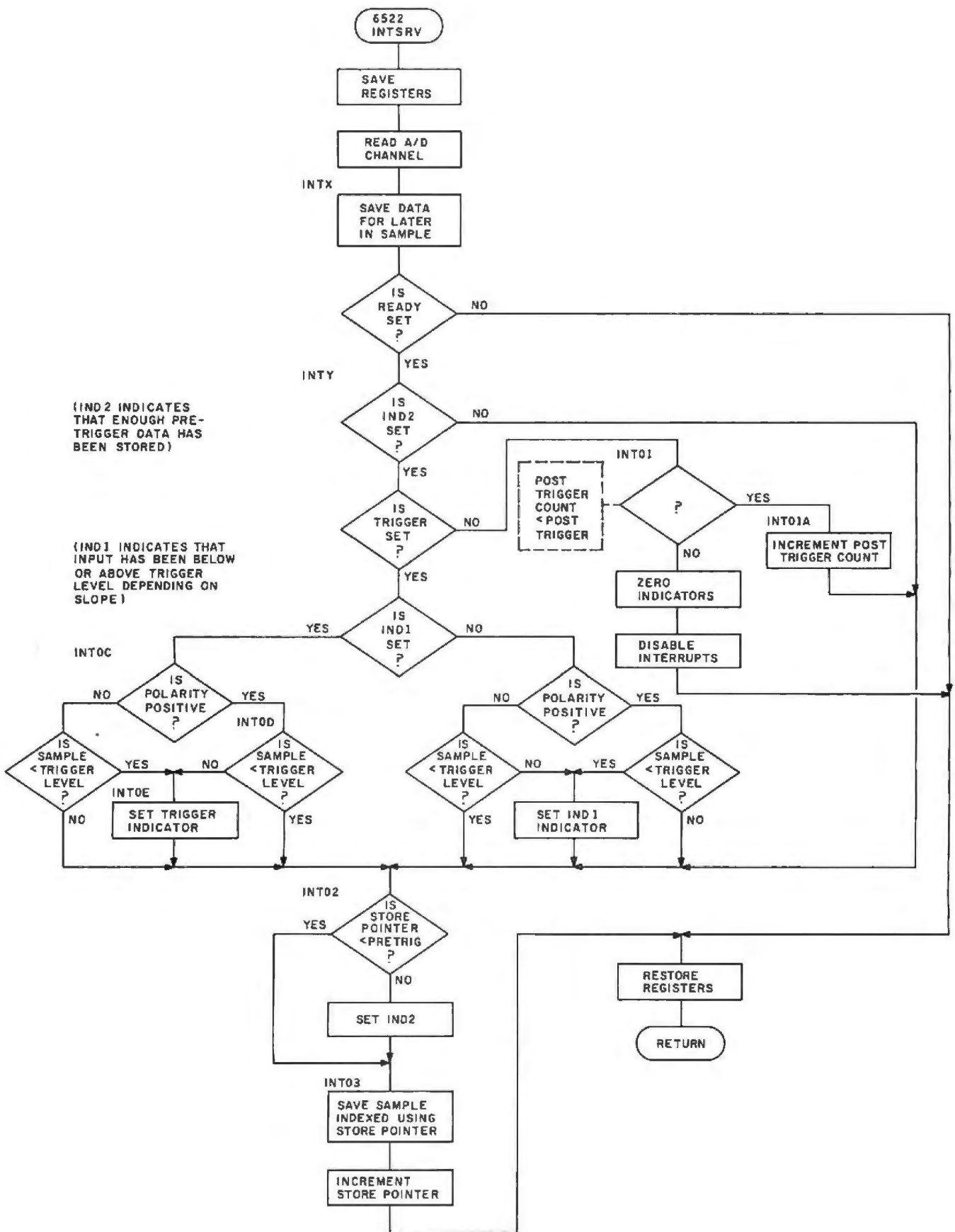
Figure 3: Flowchart of the interrupt-service routine within Adcode (see listing 1b). This routine stores data in Array2 until the trigger conditions are met and the post-trigger samples are accumulated.
