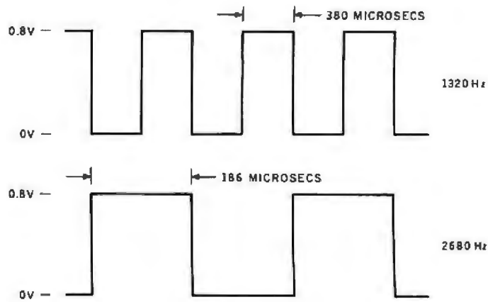
Figure 2: The 1500-bps tape format for the Model III uses a frequency-shift-keying technique. Two frequencies are used to represent 0s or 1s.
