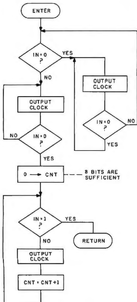
Figure 14: The ADC algorithm is straightforward. Starting from a known condition, the cassette input is sampled and the clock pulses are counted until the analog input voltage falls below the ramp voltage.
