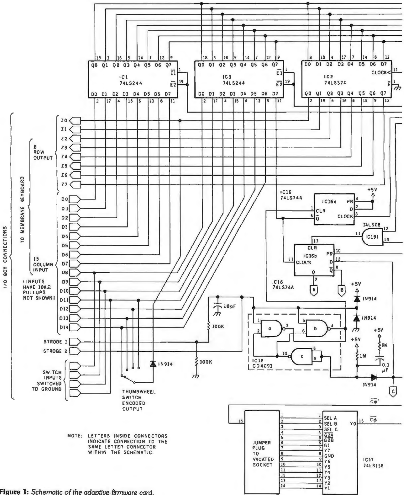
Figure 1: Schematic of the adaptive firmware card.
