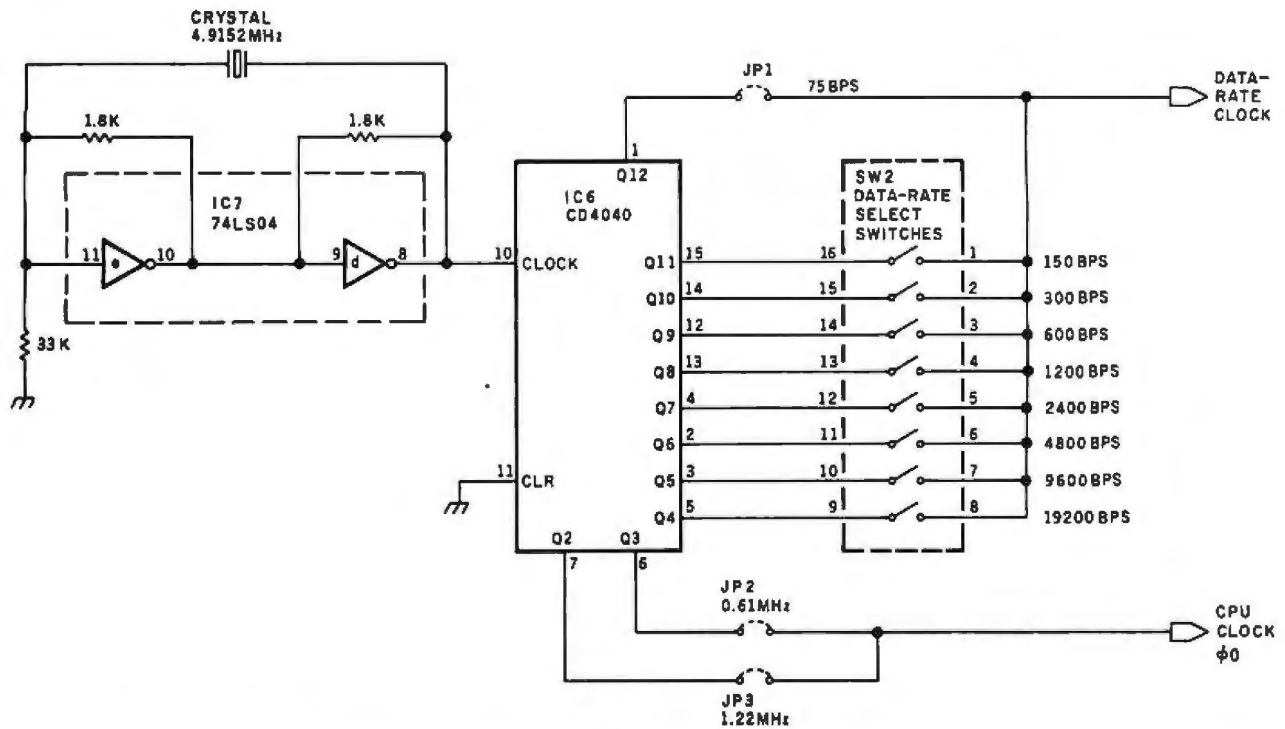
Figure 4: A detail from the Microvox circuit, showing the circuitry that derives the data-rate and clock frequencies. With this simple, low-cost arrangement, all standard data rates, except 110 bps (bits per second) and 134.5 bps, are available. Also, a trade-off must be made in selecting a clock rate for operating the microprocessor.
