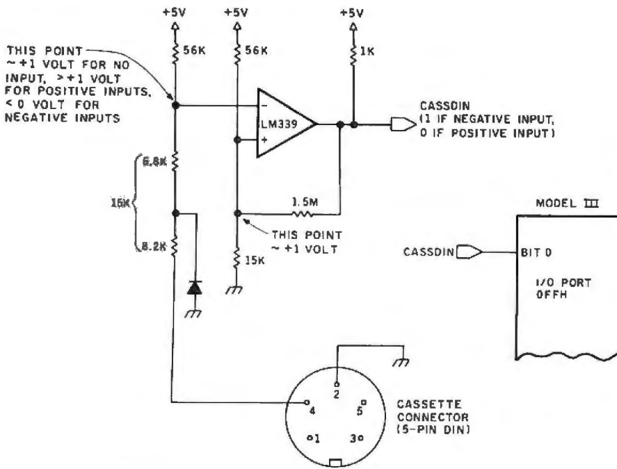
Figure 4: The Model III cassette input logic for 1500 bps uses a zero-crossing detector to detect when the input waveform goes negative. The output of the comparator goes to bit 0 of input port hexadecimal FF.
