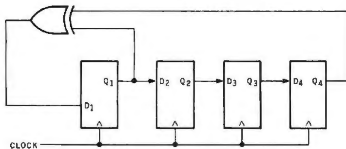
Figure 2: Model pseudorandom binary-number generator. This circuit produces the sequence of binary numbers shown in table 1, with just a simple shift register and an Exclusive OR gate.
