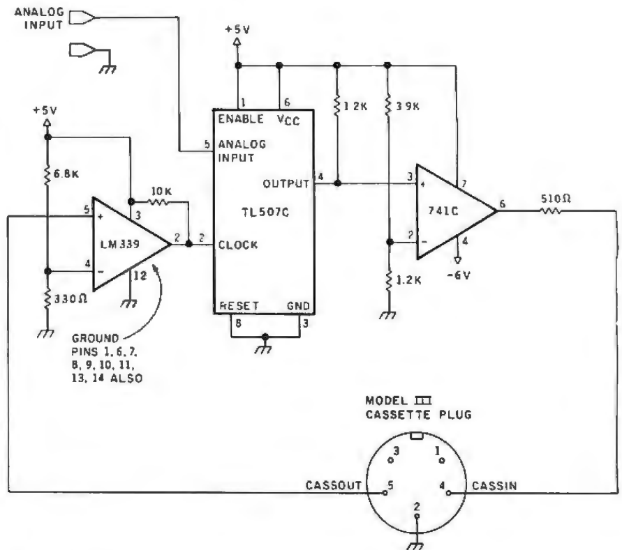
Figure 9: Three chips make up the ADC circuit that connects to the cassette jack of the Model III. The TL507C is the heart of the ADC, and the remaining chips perform level conversion.
