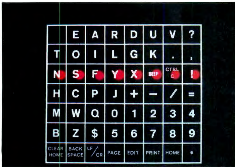
Photo 4: The optimized scanning array of the TIC is arranged according to the frequency of letters in the English language.
