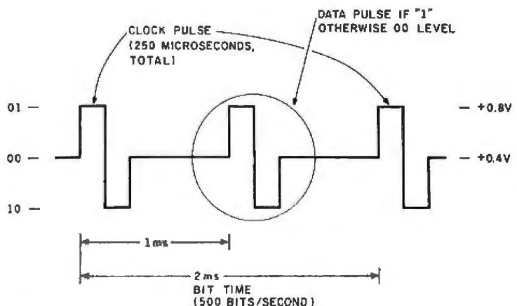
Figure 1: The 500-bps tape format of the Model III (and Model I) uses a clock pulse and data pulse for each data bit. The data pulse is absent for a 0 bit.
