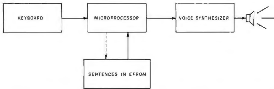
Figure 1: The bulk of the Minspeak's memory is erasable programmable read-only memory (EPROM). The voice synthesizer used in the first prototype was the Votrax SC-01.
