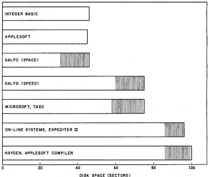
Figure 2: Comparison of disk storage requirements for a version of the Yahtzee game, using the two interpreted BASICs and four of the five compilers. Shaded segments of the bars represent the run-time libraries required by each system. Both the fastest-execution and the minimum-program-size options for Galfo Systems' Integer BASIC Compiler are shown. As described in the text, the test program was too long to be compiled by Speed Star.
