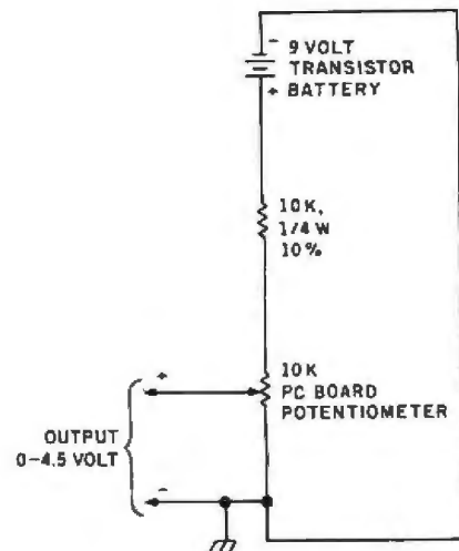
Figure 13: The ADC may be tested by a simple voltage divider made from a 9-V transistor battery, a 10k-ohm resistor, and a 10k-ohm printed-circuit-board potentiometer.
