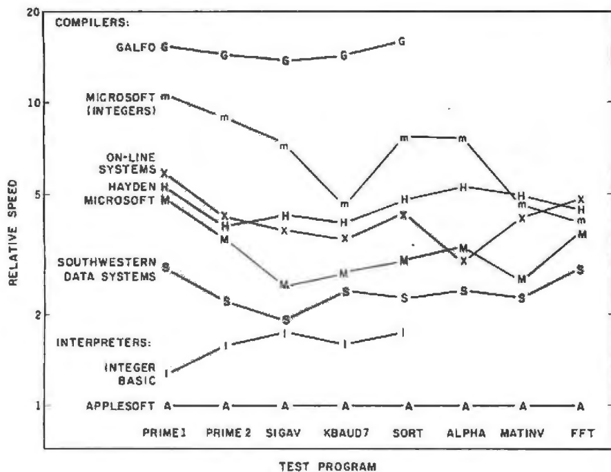
Figure 1: Relative speed of eight test programs when run directly with the Apple computer interpreters and after compiling them with each of five compilers. The speeds are normalized to a value of 1.0 for the Applesoft interpreter. Two sets of data are given for the Microsoft compiler; those denoted by lowercase m were obtained by including an Integer declaration for all numeric variables used as integers.
