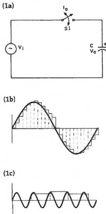
Figure 1: The sampling concept. Figure 1a shows a simple arrangement for sampling. Figures 1b and 1c compare the results of sampling at high and low rates. Sampling at a rate less than twice the frequency of the input signal (figure 1c) produces a type of error called aliasing.
