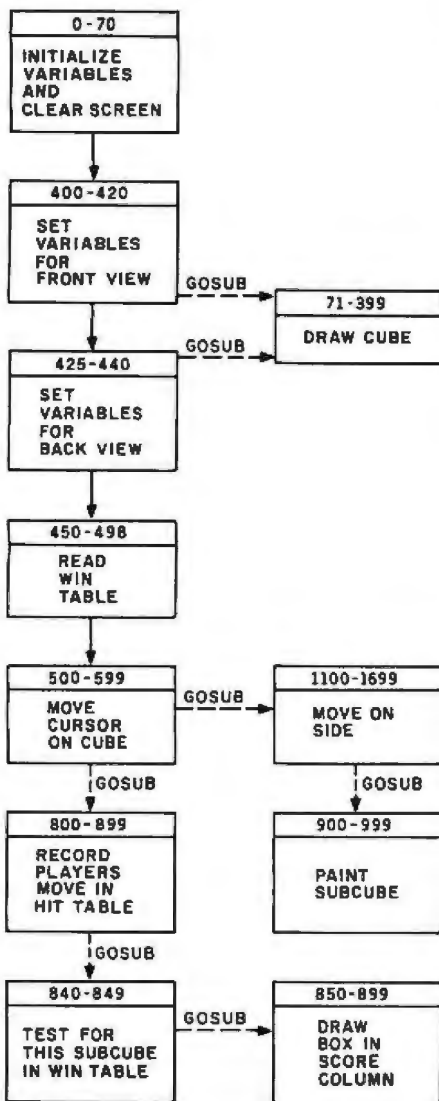
Figure 2: Flowchart of the Three Dee Tee program.
