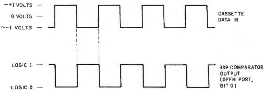
Figure 5: The cassette input waveform is a nominal 2 V peak to peak. The resulting output from the comparator is an inverted duplicate.
