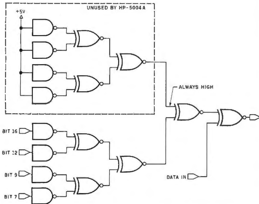
Figure 4: Two methods of using a four-input Exclusive OR device. Figure 4a is the equivalent of figure 3, with the internal architecture displayed. Figure 4b shows the insides of the 82562 device used by Hewlett-Packard.
