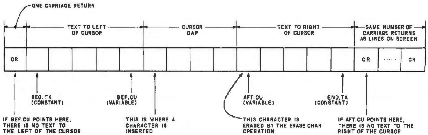
Figure 2: The structure of the text as stored in memory. Carriage returns are added to the ends of the text area to simplify the editor program, but they are not considered part of the text. The available text area extends from BEG. TX to END. TX , but the BEF. CU and AFT. CU pointers indicate how much of this area contains text; the unused portion constitutes the "cursor gap." The text code used for characters (except spaces) and carriage returns is ASCII, with the eighth bit set to 1. Spaces are represented when the eighth bit is set to 0, in which case the other 7 bits indicate the number of adjacent spaces stored at that location. In this diagram, memory-address numbers increase to the right.
