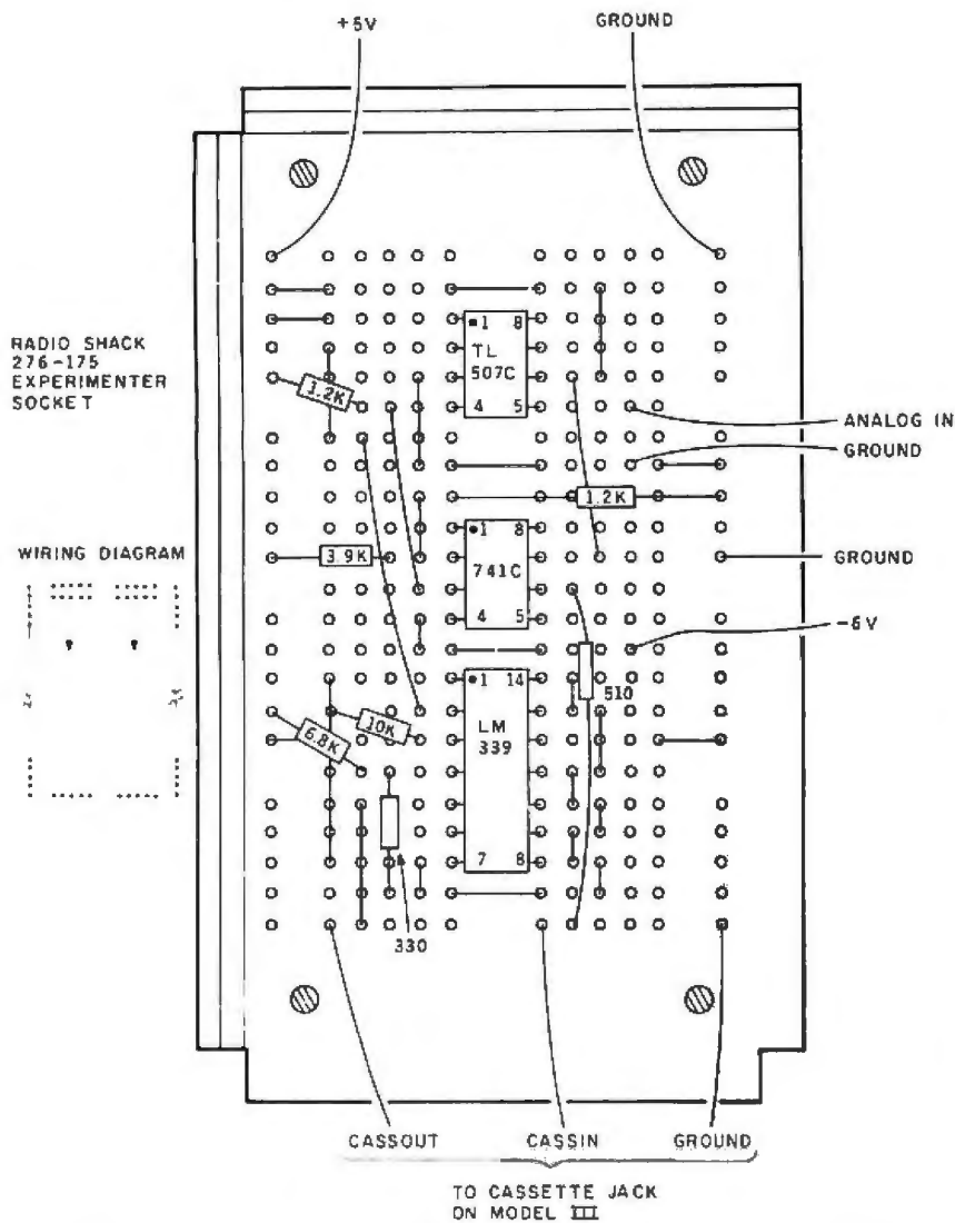
Figure 11: The simple and inexpensive ADC is constructed on a Radio Shack 276-175 prototype board.
