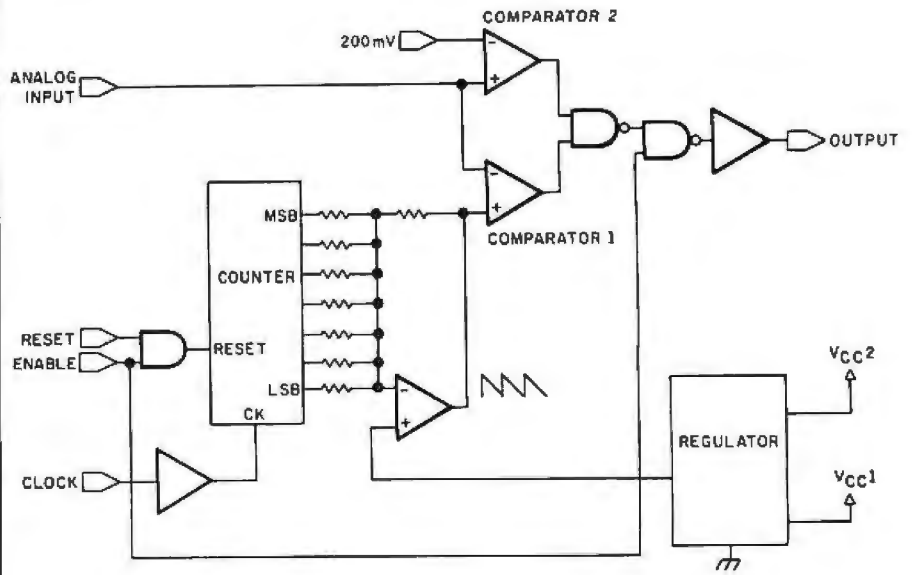
Figure 6: The TL507C chip is an analog-to-digital converter (ADC) that compares an analog input to an internally generated ramp voltage that steps through the allowable range of input voltages. The comparator output goes true when the ramp voltage falls beneath the analog input voltage.
