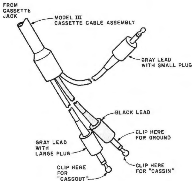
Figure 12: The existing cassette cable for the Model III may be used to connect the ADC to the computer system. Three clip leads connect all signals.
