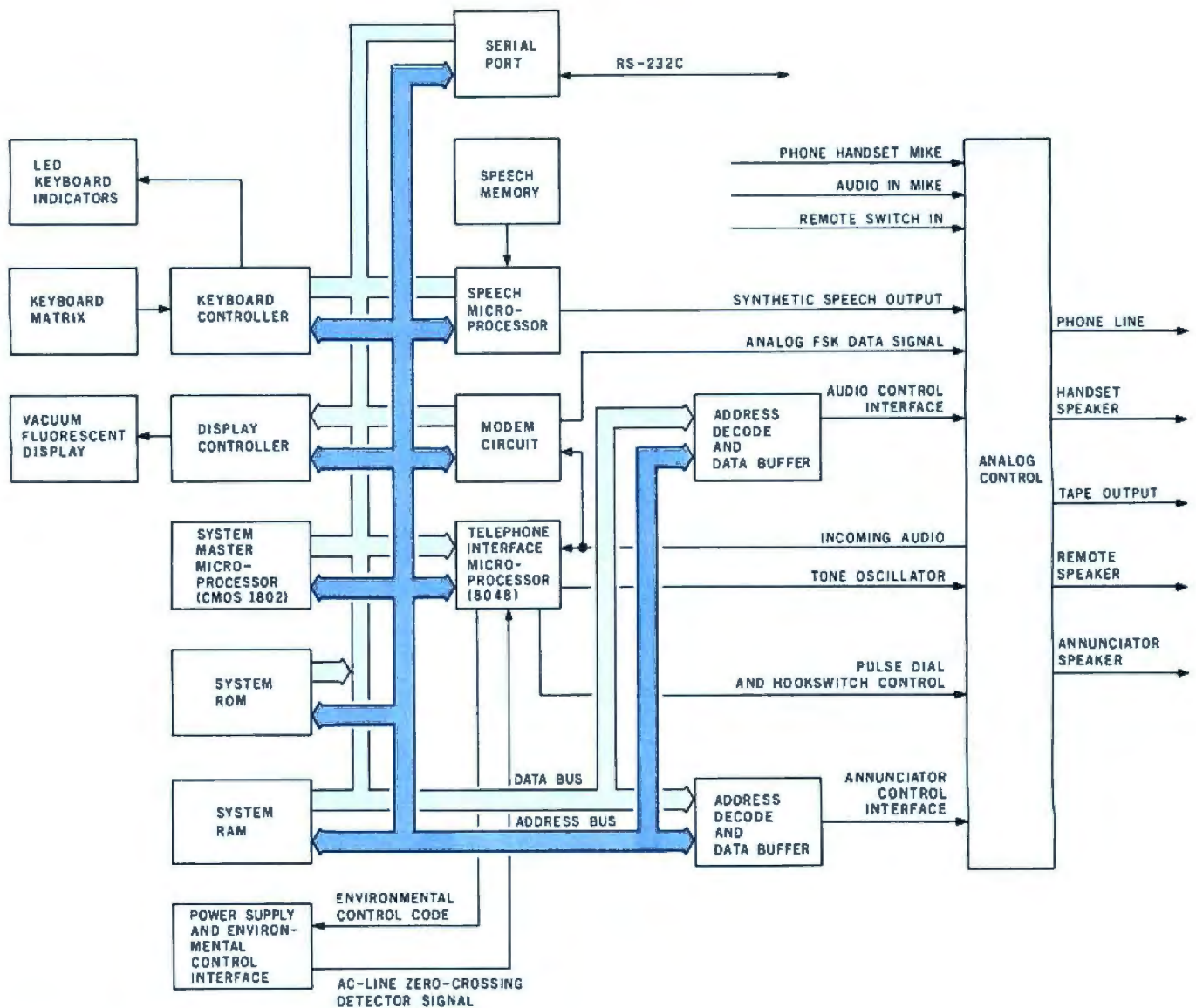
Figure 1: A block diagram of the Abilityphone.
