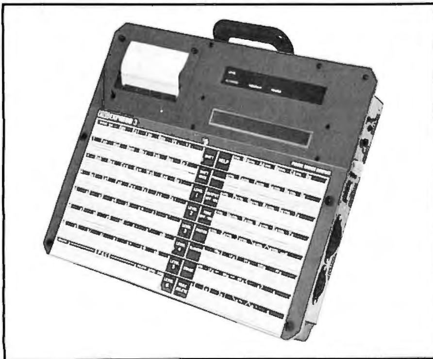
Photo 2: The Express 3, developed by Prentke Romich Co., is a portable communication aid powered by internal rechargeable batteries and designed for mounting on a wheelchair. A special Express 3 is being prepared to implement the Minspeak concept. The system will use a combination of power-strobed EPROM and CMOS RAM. A Votrax Speech PAC with an SC-01 voice synthesizer marketed by Vortex will be coupled to the output of the microprocessor. It will retain other features of the original Express 3, including a 40-character upper- and lowercase liquid-crystal display with corresponding thermal printer and serial ASCII output for connection to other computers and environmental-control devices.
