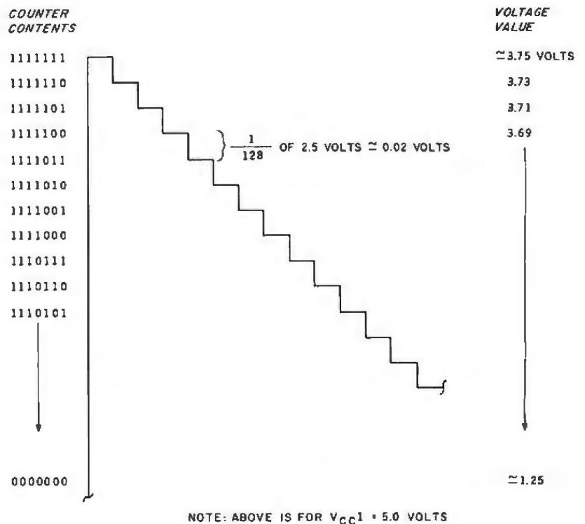
Figure 7: The TL507C generates a ramp of voltages from a 7-bit counter and a "weighted" resistor network. The smallest increment is 1/128 of the total voltage range for the ramp.
