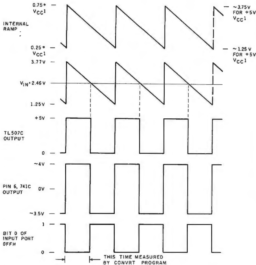
Figure 8: The analog-to-digital conversion is performed externally to the TL507C by measuring the duty cycle of the chip's waveform output. The duty cycle changes according to the analog input voltage.
