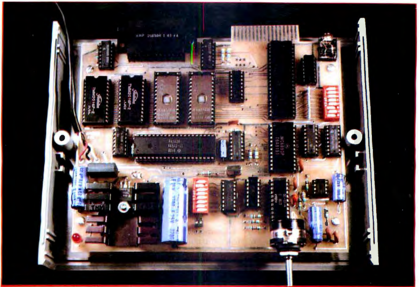
Photo 1: Prototype of the Microvox speech synthesizer, which can pronounce texts consisting of English words from their representation as ASCII characters according to fixed pronunciation rules. The Microvox contains a general-purpose 6502-based microcomputer programmed to control the Votrax SC-01A-based speech-synthesis circuitry.
