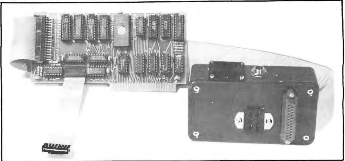
Photo 1: The adaptive-firmware card. The device allows disabled users to run standard, unmodified software (such as games, Visicalc, Easywriter, etc.) using any of 10 input routines, some of which require use of only a single switch. (Photo by Ed Crabtree.)
