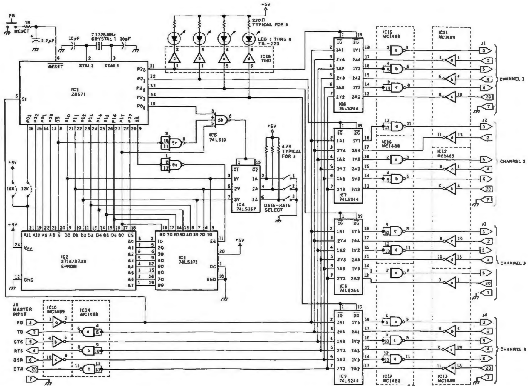
Figure 2: Schematic diagram of the Micromux prototype four-channel code-activated switch. This design uses a Z8671 as a controller to monitor codes embedded in the transmitted data and activate the appropriate signal buffer for the channel. Only the six
