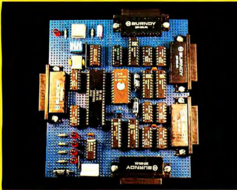
Photo 1: Prototype of the Micromux four-channel code-activated switch, built around a Zilog Z8 single-chip microcomputer.
