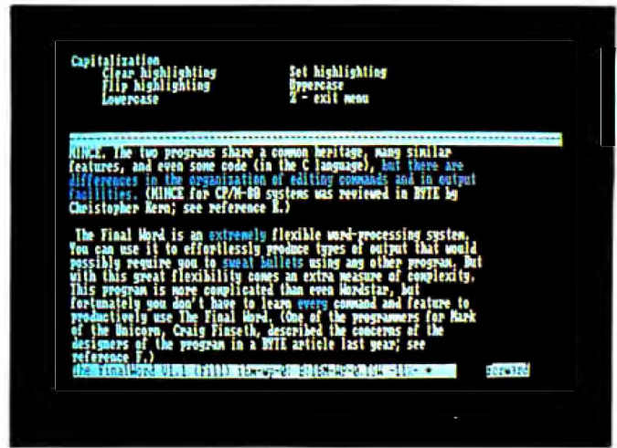
Photo 13: When you type Control-X, a top-level menu of menus appears at the top of the screen. You then type a character (control or regular) to select one of the menu choices, such as the menu of Capitalization commands shown here. You then hit one more key to invoke the desired operation.
