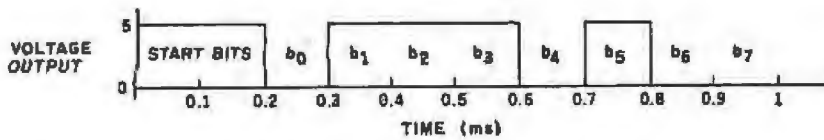
Figure 4: Diagram of the serial bit stream generated by the IBM PC keyboard when a key is pressed. The graph shows the voltage output (pin 2) versus time, starting when the C key (code 46 decimal, or 00101110 binary) is pressed. The voltage levels are TTL-compatible. In the absence of transmission, the keyboard sends a 0-V level. Two +5-V (high) "start bits" define the start of a character. Eight bits follow, each lasting 0.1 ms, except for the last, which is slightly shorter.
