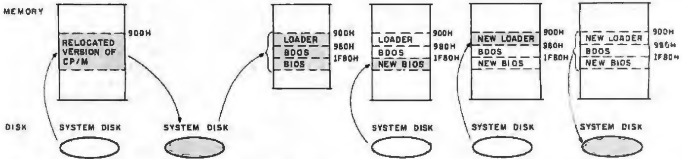
Figure 6: Installing the new operating system. First, the MOVCPM instruction reads the current version of CP/M from the disk into memory at location 900 hexadecimal and relocates it to run at a location specified in the command. The SAVE instruction then places the relocated version of CP/M onto the disk under the filename CPMNN.COM. The DDT command reloads the relocated version of CP/M into memory at location 900 hexadecimal and transfers control to the DDT program. Next, the command I NEWBIOS.HEX reads the new BIOS from the disk and overlays the existing BIOS. The command I NEWLDR.HEX then reads the new system loader from the disk and overlays the existing loader. Finally, the WRITE utility program writes the properly configured operating system to the first track of the Winchester disk.
