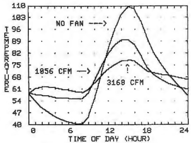
Figure 4: Tswing enables a user to test the effect of various parameters such as airflow rate on a solar design.
