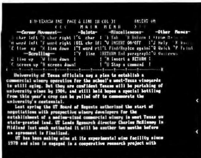
Photo 9: A typical editing screen display produced by Wordstar. Status information is displayed on the top line of the screen; the menu occupies the next several lines. Below the menu is the tab and margin ruler.
