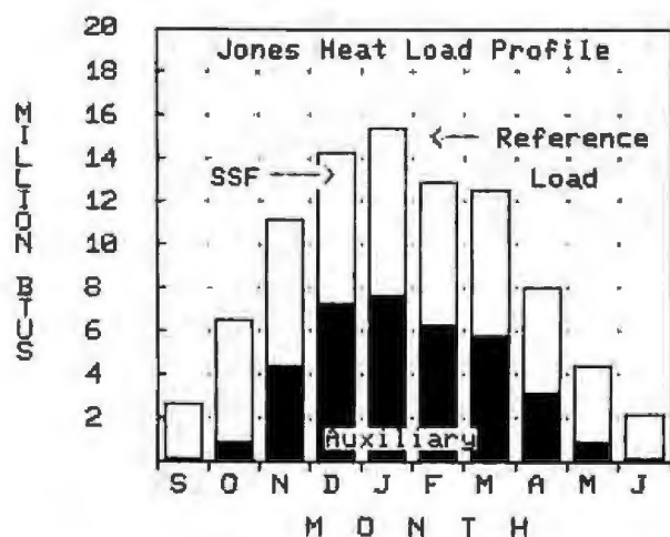
Figure 1: Sunpas can produce a bar chart of the monthly auxiliary heating load and solar saving fraction.
