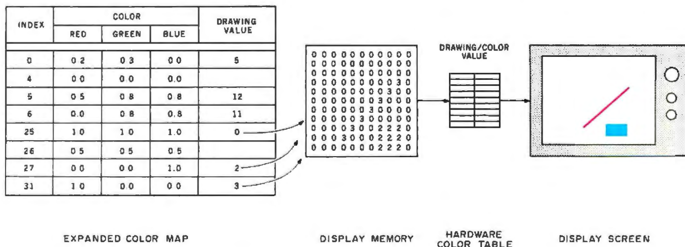
Figure 3: A typical color-table implementation. Note that special color-map hardware is required. The drawing value is the one used when drawing occurs in the display memory. It is an index into the hardware-based color map.
