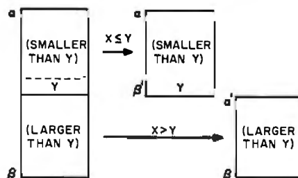
Figure 1: A simple comparison reduces the problem of searching for x in a sorted array (left) to searching for x in a sorted array half the size of the original (right).
