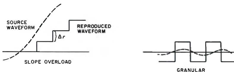
Figure 3b: Two potential problems occurring in delta modulation. When the source waveform changes too rapidly, the fixed quantization value may be too small to express the full change in the input; this slope overload causes a compliance error. Or when there is little change in the input waveform (at the extreme, a DC signal), vertical deflection in the quantization value results in granular noise in the output.
