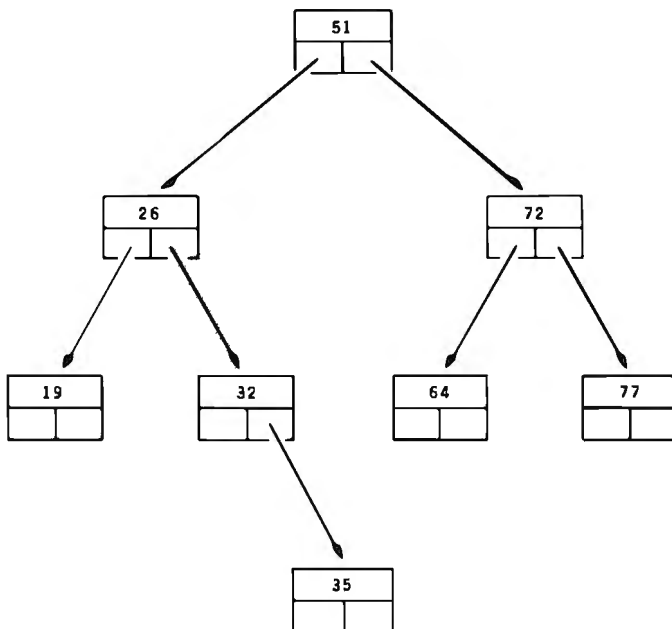
Figure 4: Inserting a new entry into a tree creates a new level.
