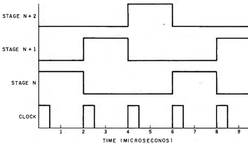
Figure 2: As illustrated in this timing diagram showing the figure 1 circuit's clock signal and three register-stage outputs, sequencer data remains stable for about 1.5 \mu s following a negative-going clock transition.
