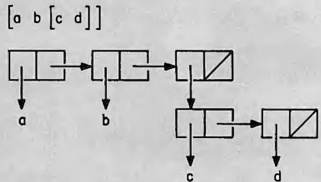
Figure 1: The list containing the two atoms "a and "b and the list [c d] is shown above in its node representation. Each node consists of two 2-byte fields that can be used as data or pointers to more data.
