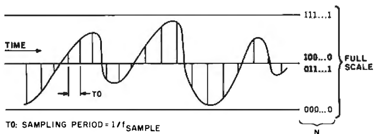
Figure 2: Waveform sampling by pulse-code modulation (PCM). The interval between samples is T_0 ; the sampling frequency is the reciprocal of the interval. Each sample of PCM data consists of N bits; the leftmost is the most significant bit and the rightmost is the least significant bit.
