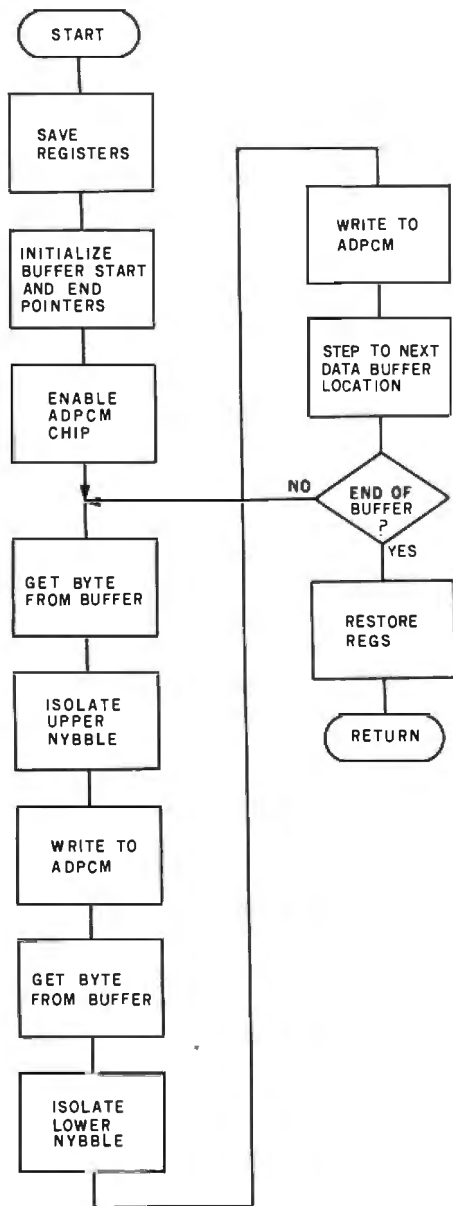
Figure 9: Algorithm of the DUMP routine from listing 1. This routine takes the stored ADPCM-encoded speech from memory and causes the circuit of figure 7 to reconstruct the voice waveforms.
