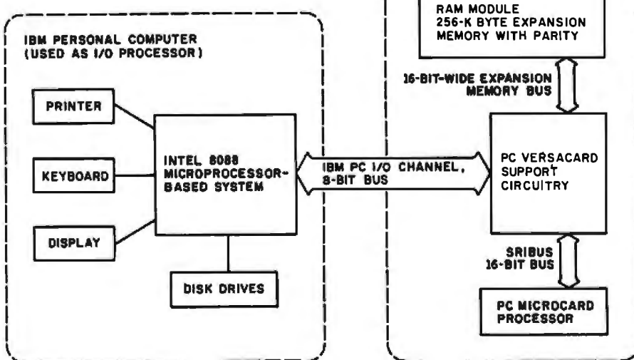
Figure 1: Architecture and mechanical arrangement of the Versacard. The extra memory and the additional processor plug into the Versacard (figure 1a), so that the whole unit requires only one IBM expansion slot. The architecture of the complete system, including the IBM PC, is shown in figure 1b.
