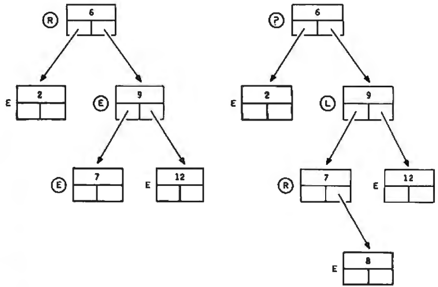
Figure 7: Inserting a new element in a tree (left) requires changing the balance factors.
