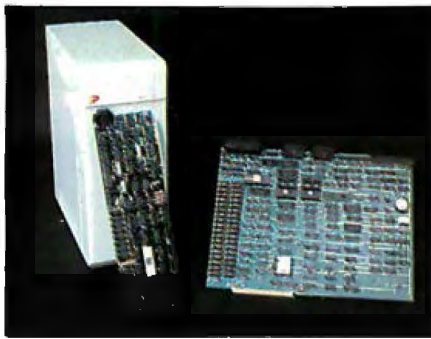
Photo 2: The graphics adapter of the Pronto Series 16 leaning against the system housing, and large main system card.
