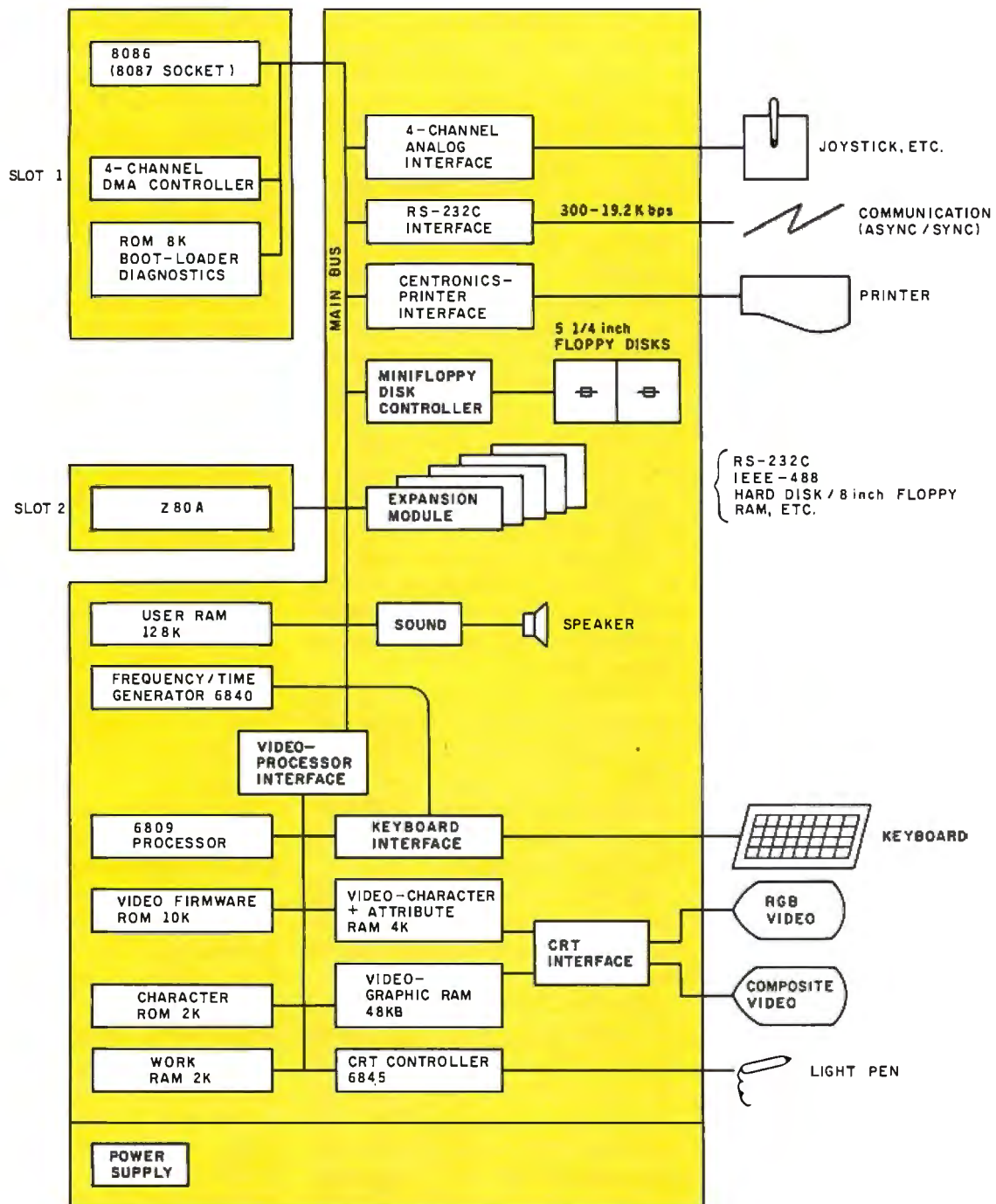
Figure 2: A block diagram of the Micro 16s system. The 8086 processor is plugged into slot 1 and the Z80A into slot 2.
