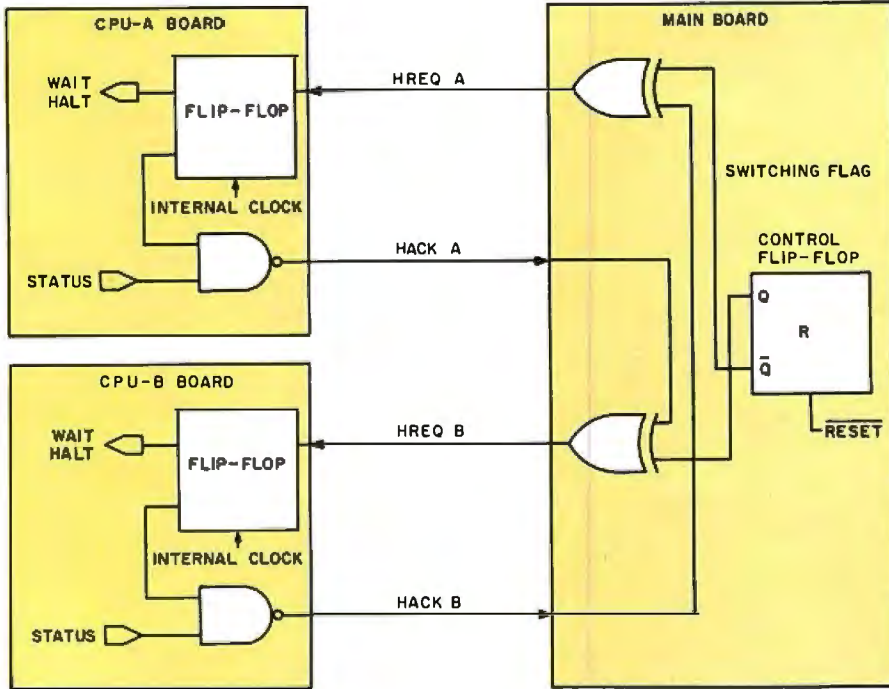
Figure 3: A simplified diagram showing how control is transferred from one processor to another. The control flip-flop on the main board can be set under program control. When this happens, a halt-request signal is sent to the operating processor, which then sends a halt-acknowledge (HACK) signal, which then gives the other processor control. The HREQA, HACKA, HREQB, and HACKB signals are on the Fujitsu 130-pin bus. CPU-A refers to the processor in slot 1; CPU-B, the processor in slot 2.
