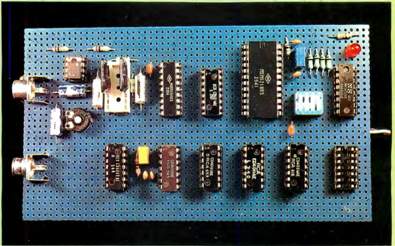
Photo 2: Prototype of the speech analysis and synthesis circuit of figure 7, built around the Oki Semiconductor MSM5218RS integrated circuit. The empty IC socket is used for ribbon-cable connection to the host computer.
