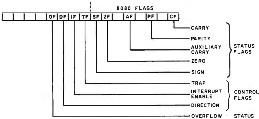
Figure 2: The 8086 has six 1-bit status flags and three control flags in a 16-bit word register, with its low byte identical to the 8080 flag register.
