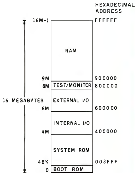
Figure 2: Memory map for the Model 16.
