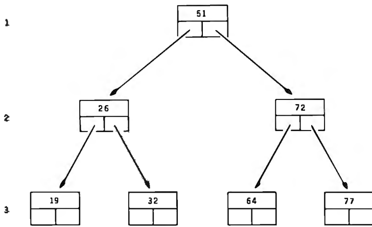
Figure 2: An AVL tree represents sorted data as interlinked nodes.
