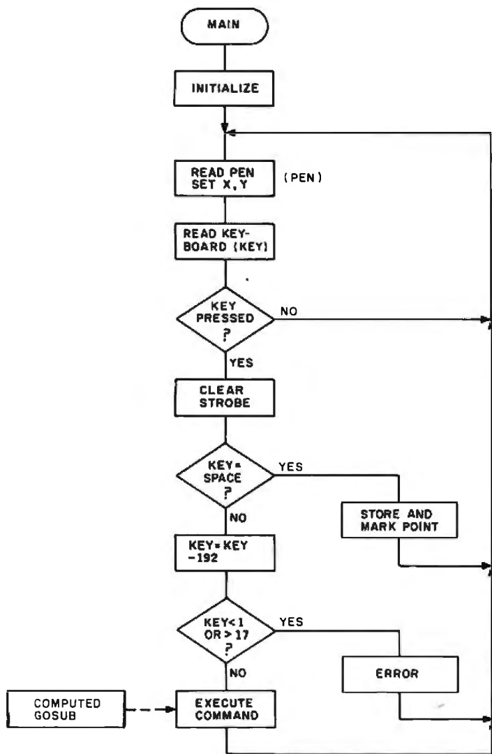
Figure 3: Outlining the course of the LINES program, this flowchart lists the steps you take to use the light pen to draw figures on the screen.
