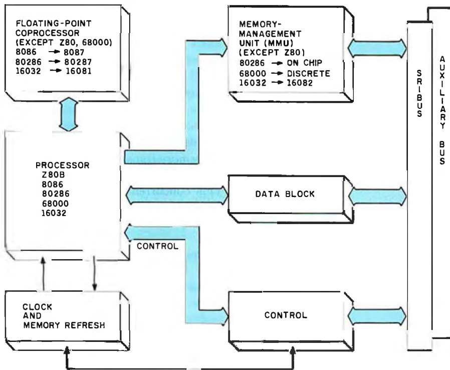
Figure 2: Architecture of the Microcard.
