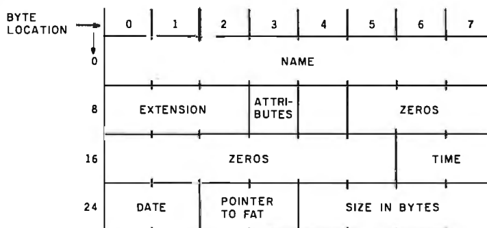
Figure 3: Arrangement of bytes in disk directory entry.
