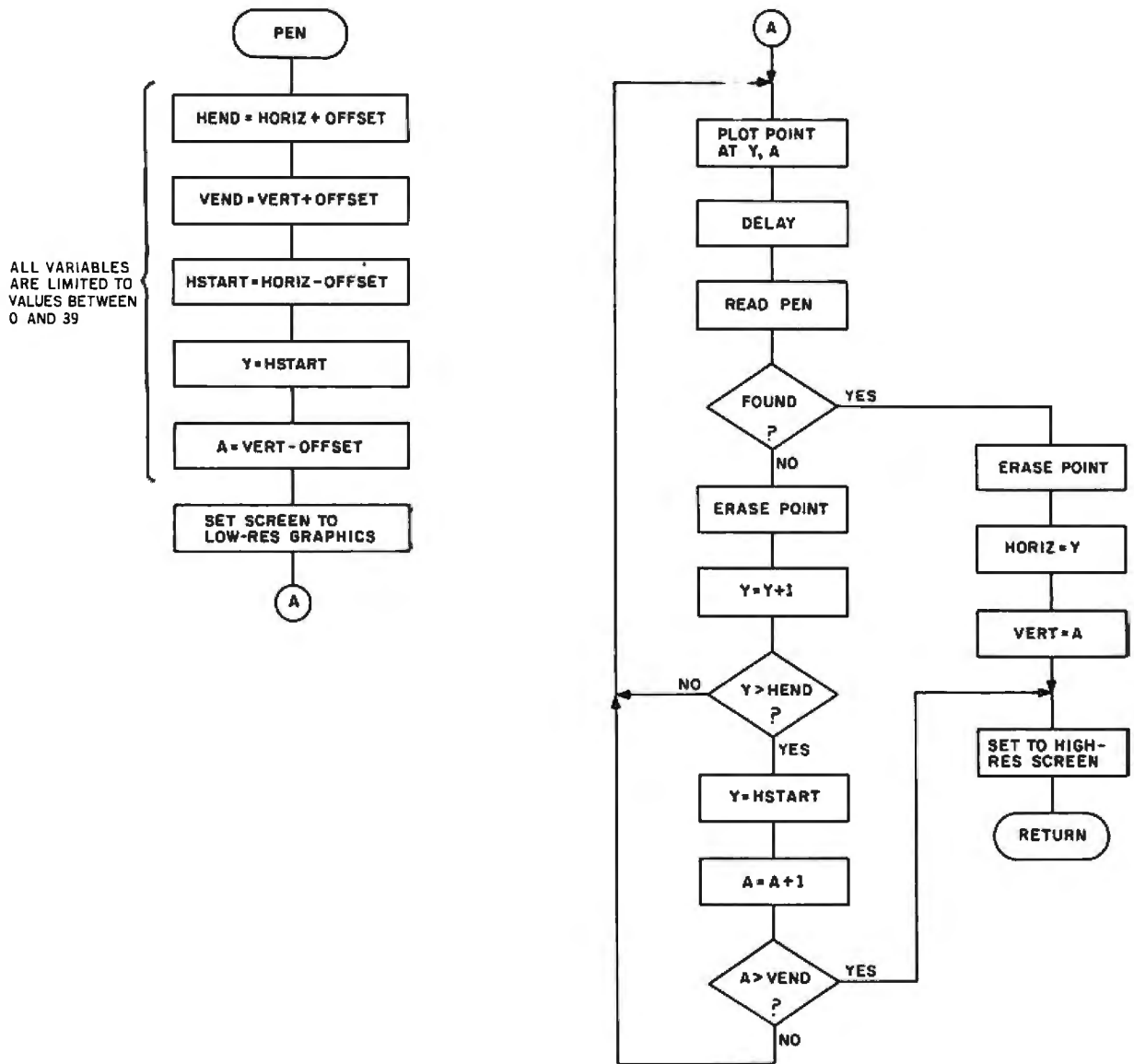
Figure 2: This flowchart plots the course of the PEN subroutine, which uses the top portion of the low-res display.
