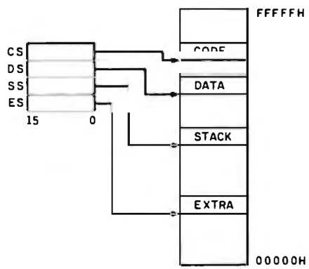
Figure 3: The four segment registers contain the base address, or beginning location, of the current code, data, stack, and extra data segments.
