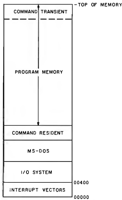
Figure 1: Map of memory areas as assigned by MS-DOS.
