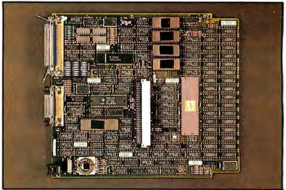
Photo 3: One of the most tightly packed boards in the microcomputer industry. The main processor board of the Model 16 is only 9 by 10.3 inches but contains 125 special integrated circuit chips, the equivalent of 185 normal (14- to 18-pin) chips. The result is a chip density equivalent to approximately 2 chips per square inch.
