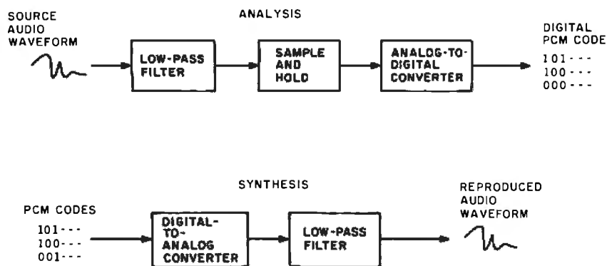
Figure 1: Functional block diagram of a digitized speech-reproduction system that employs pulse-code modulation.
