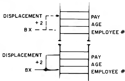
Figure 8: A record of dissimilar items uses a base register to point to the beginning of the record, with the displacement pointing to the item needed. The base can be re-adjusted to point to the base of a new record with the same displacement to access an item in the same position.
