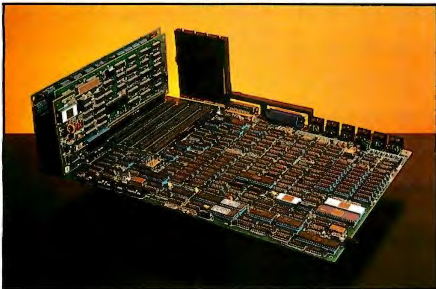
Photo 2: The main circuit board of the Fujitsu Micro 16s. Two processor boards are plugged into the expansion slots.
