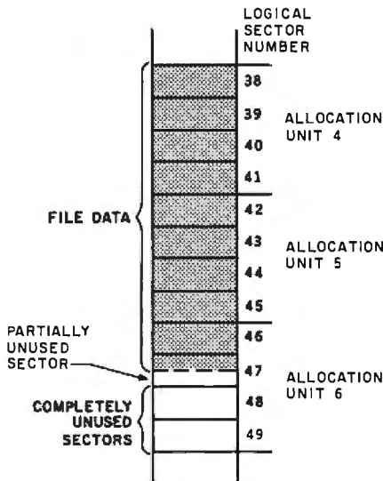
Figure 4: Assignment of logical sectors to allocation units. Note that, in the file shown, more than two sectors are wasted because they are in an unused part of the last allocation unit.
