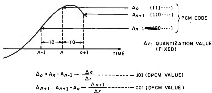
Figure 4: Differential pulse-code modulation (DPCM) is an attempt to reduce the amount of data stored or transmitted, as compared with regular PCM. For each sample, the difference between the previous PCM code and the current code is expressed in terms of a fixed quantization value \Delta r (delta-r), which must be chosen with attention to the characteristics of the source waveform. If too large or small a quantization value is used, compliance errors occur.
