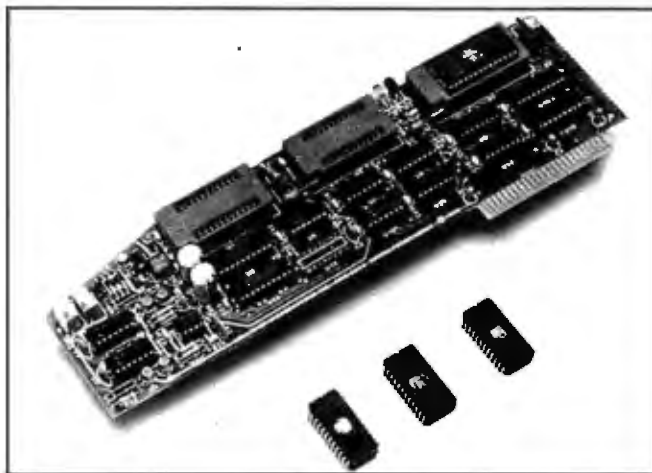
Photo 1: The HMS3264 programmer card for the Apple II.
