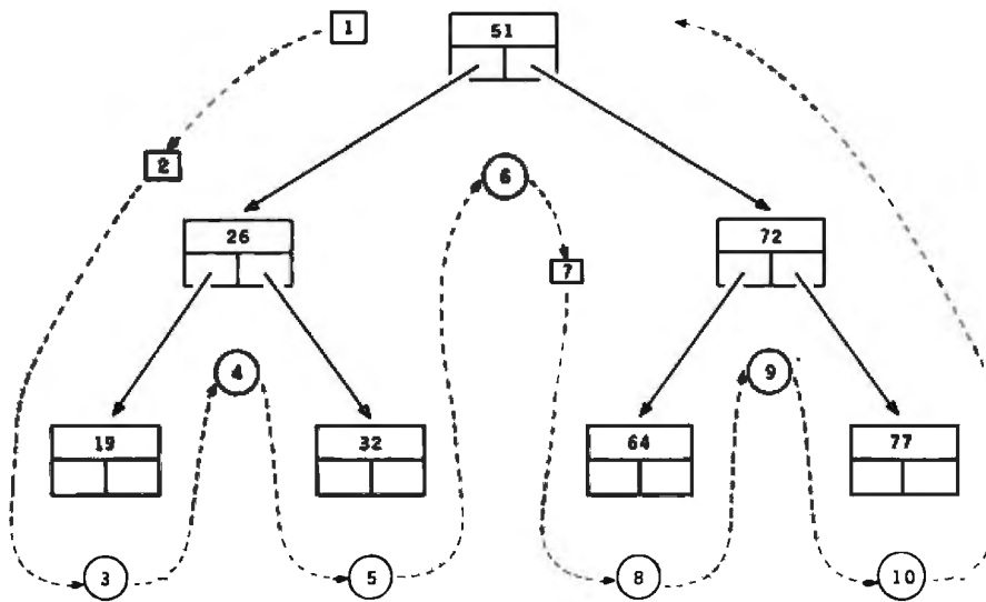
Figure 3: To print an AVL tree in sorted order the computer traverses the tree along the path shown. The circled numbers indicate points at which elements are printed.
