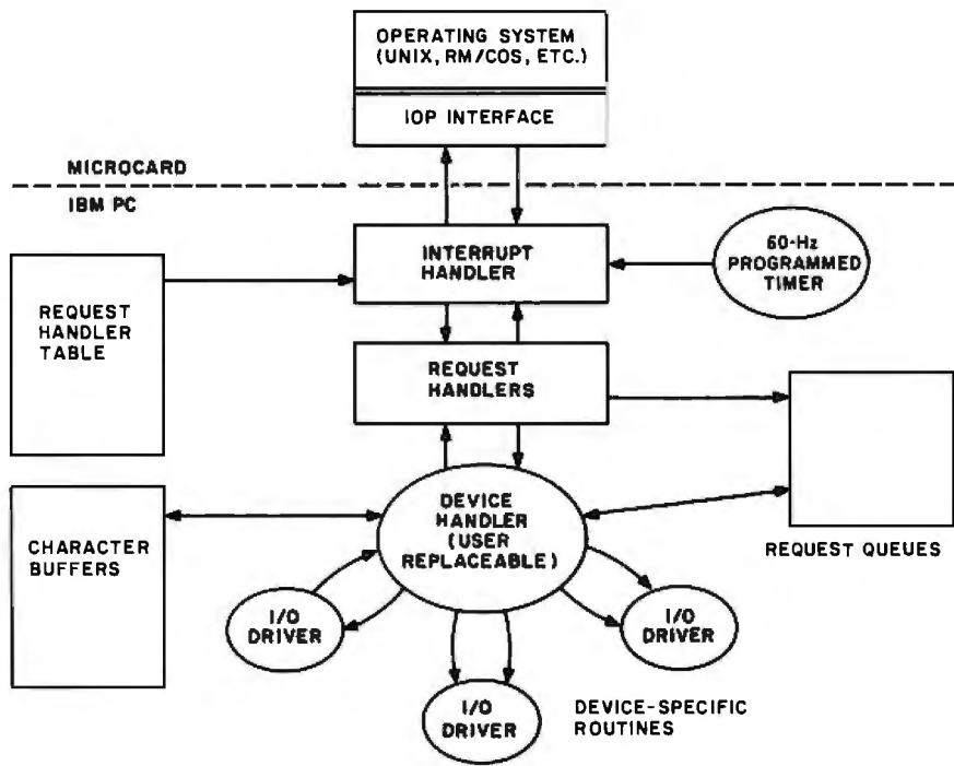
Figure 3: Flow diagram of the I/O Processor software.
