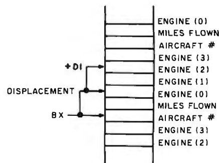
Figure 9: The base register points to the beginning of the record containing the array, the displacement points to the beginning of the array, and the index points to the item needed.
