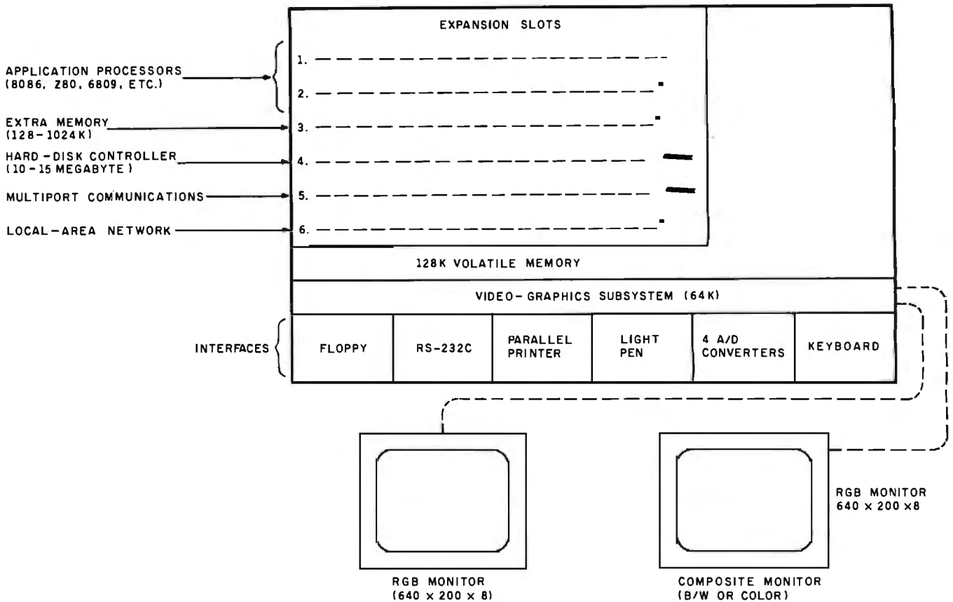
Figure 1: Diagram of the Fujitsu Micro 16s computer. Two applications processors (the 8086 and the Z80A) come standard with the unit along with an RGB monitor and dual disk drives. The video-graphics subsystem uses a 6809 processor and has its own 64K bytes of memory. Slots 2 through 5 are identical and can house any combination of cards.
