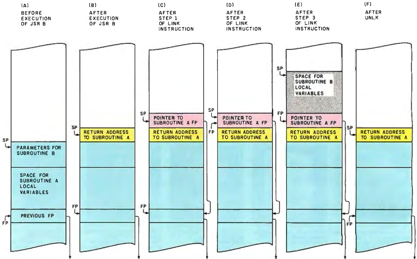
Figure 1: Use of the LINK and UNLK (unlink) instructions, both of which help the assembly-language programmer manage memory areas to be used for local variables in subroutines. See text for details.
