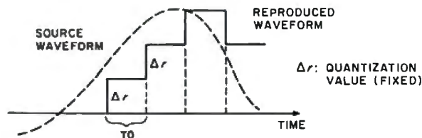
Figure 3a: Waveform sampling by delta modulation. Each sample of the source waveform is tested to see if its amplitude is higher or lower (within the resolution of a fixed quantization value \Delta r —delta-r) than that of the previous sample. If the amplitude is higher, the single-bit delta-modulated encoding value is set to 1; if lower, the encoding value is set to 0.
