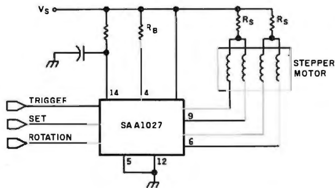
Figure 1: Stepper-motor controller.
