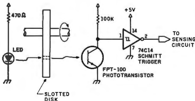
Figure 2: Position-limit sensor.
