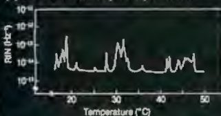
(b) With HF superimposition
