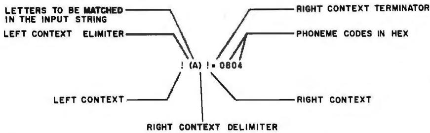
Figure 3: Format of the rules in the text-to-speech algorithm.
