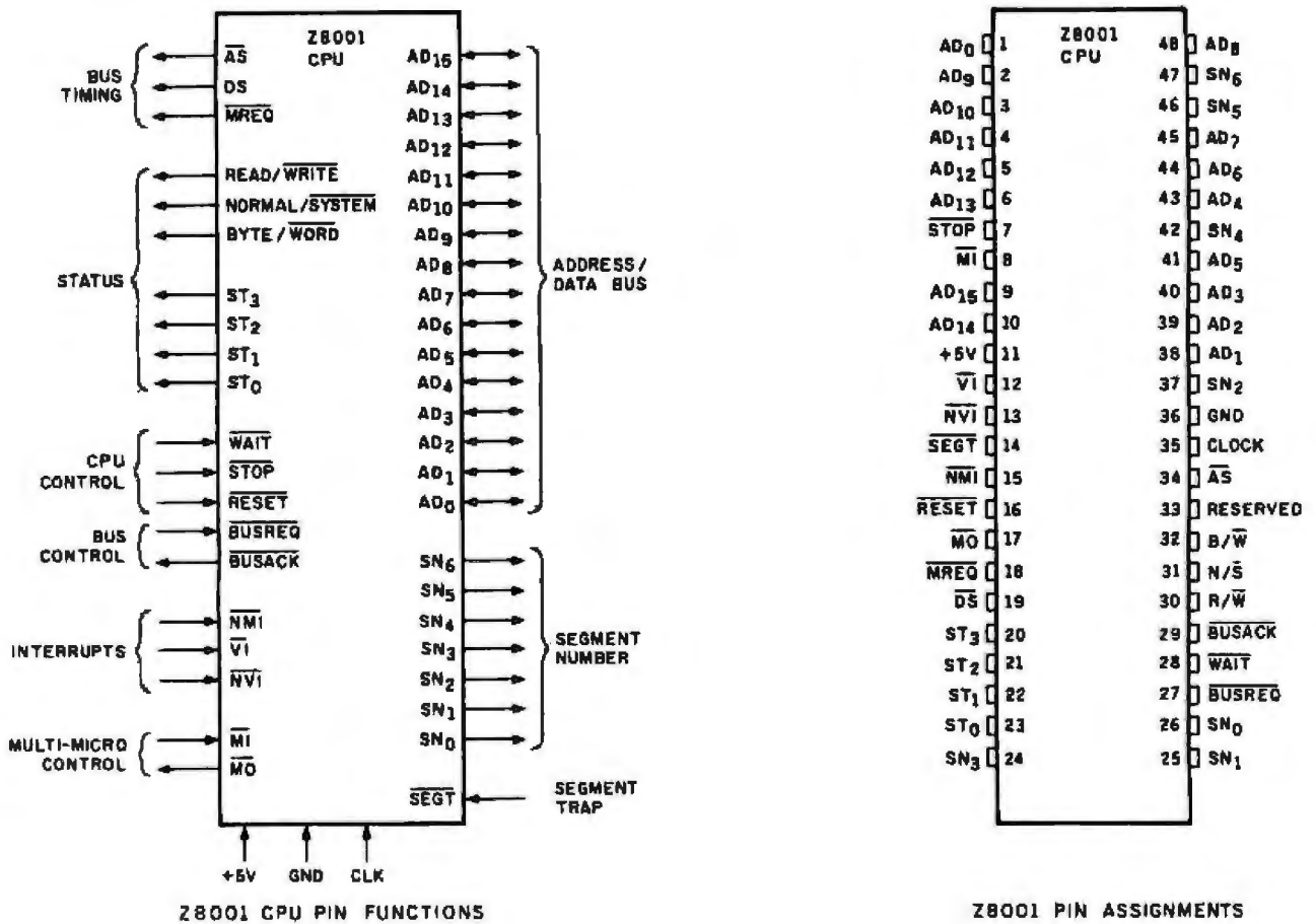
Figure 2: Pinout arrangement of the Z8001 memory-segmented version.
