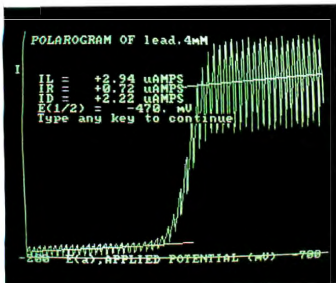
Photo 2: Students taking our analytical chemistry laboratory course analyze the amount of lead in gasoline using the interface described in the text. The diffusion current (ID on the display) is proportional to the concentration of the lead in the sample.
