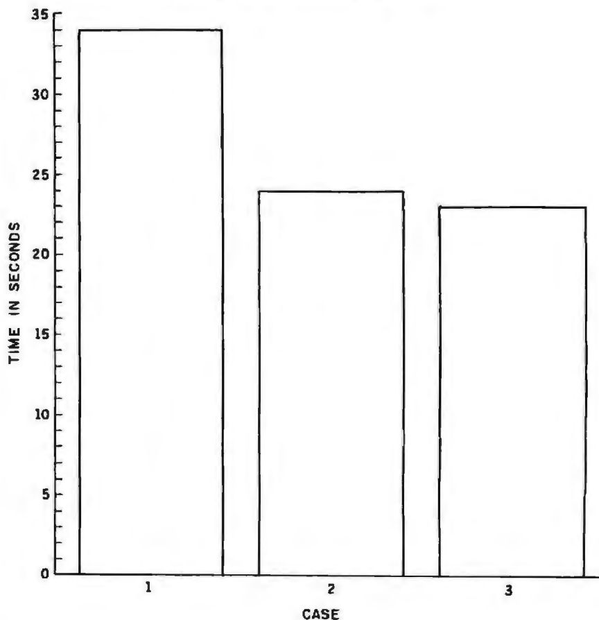
Figure 8: A bar plot of the time required to compile and link a C program. As in figure 7, bar 1 was obtained with no caching, bar 2 was obtained with an empty cache, and bar 3 was obtained with fully cached operation.
