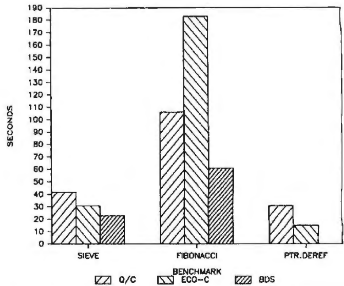
Figure 2: Comparative execution times for the various benchmarks.
