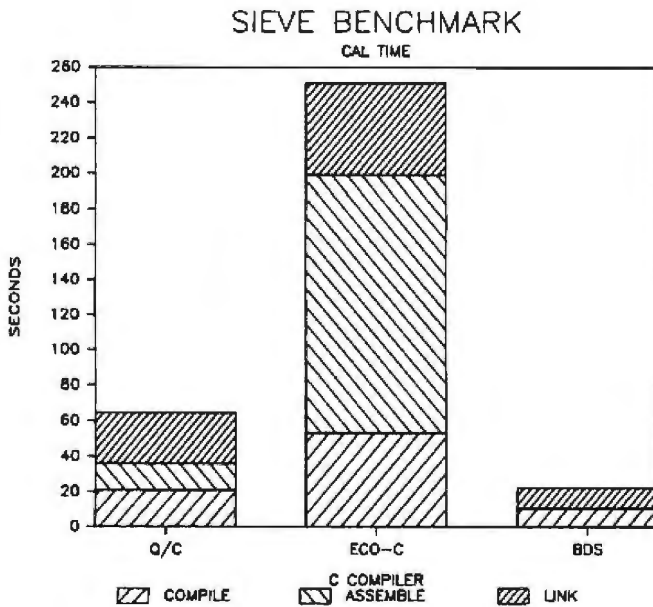
Figure 1: A comparison of the cumulative program CAL (compile, assemble, and link) times for the sieve benchmark. (All figures were drawn with a Hewlett-Packard 7475A plotter.)
