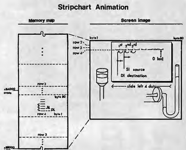
Figure 2: The chart paper is animated by overlapping string moves within video memory. Each byte is moved one position to the left; its neighbor to the right then occupies the old position. The last byte must be zeroed separately to blank the old data at that position.
