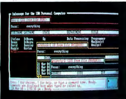
Photo 1: Scopes. Infoscope's name for windows, can be colored and then referenced by the color name rather than by the filename. On this screen, for example, the scope at top left could be moved to the cursor position with the command "move red here."
