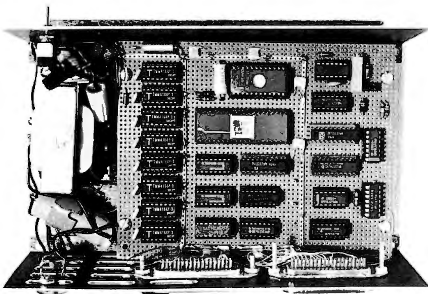
Photo 1: The inside of the completed printer buffer.
