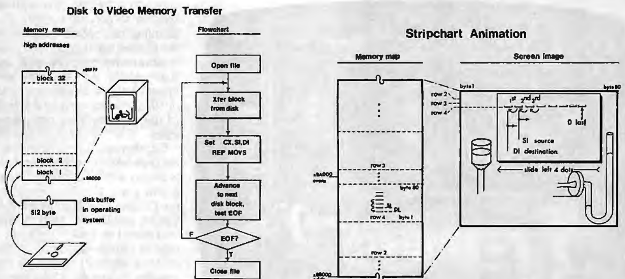
Figure 1: String moves facilitate transferring images from a disk buffer to video memory. The 8088 registers CX (counter), SI (DS) (source), and DI (ES) (destination) are involved. Whole images move in a fraction of a second from RAM or hard disk; floppy-disk drives are slower.
