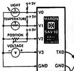
A typical SAV10 application
