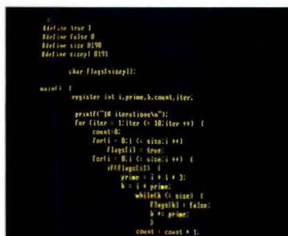
Photo 3: Programs in BASICA (3a) and in C (3b) can be written for Trump Card or the PC by using Trump Card's built-in EE editor.
