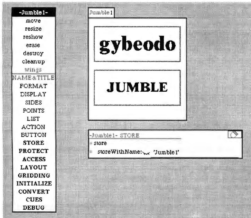
Figure 10: A stage named Jumble!; it's a category menu and cue sheet for its STORE category.
