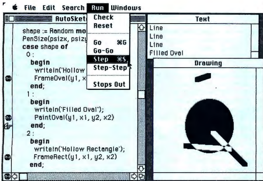
Figure 1: The Macintosh Pascal AutoSketch program. The Run menu appears in the upper center of the screen. At the right are the Text and Drawing windows. The listing window, on the left, shows breakpoints indicated by stop signs; the finger points to the next instruction to be executed in single-step mode.
