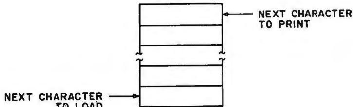
Figure 4: These diagrams show how the control software determines where to load the next character into RAM. In 4a, both pointers are equal, which indicates that the buffer is empty. In 4b, the next load position is one address less than the next print position, which means that the buffer is full. Figure 4c is a special case of the buffer-full condition in which one must compensate for the "wraparound" effect (see text).
