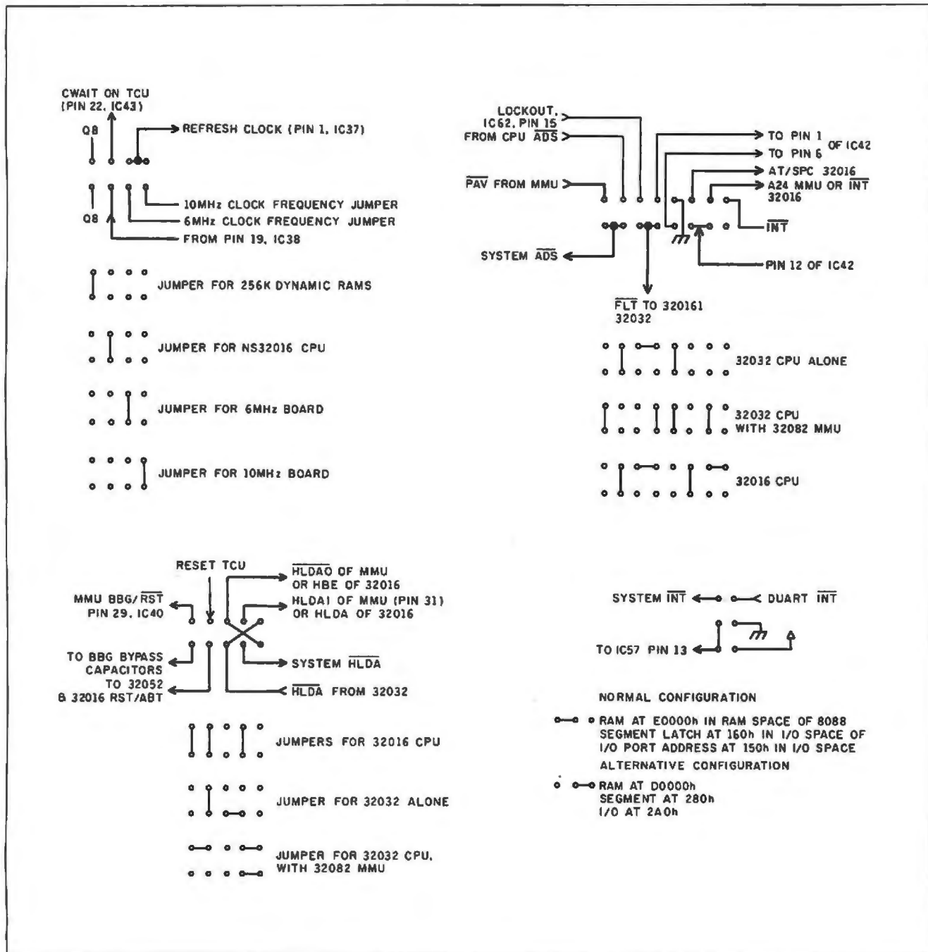
Figure 5: Various jumper configurations for the DSI-32. All diagrams are shown looking at the top of the board, with the edge connector to the bottom right.
