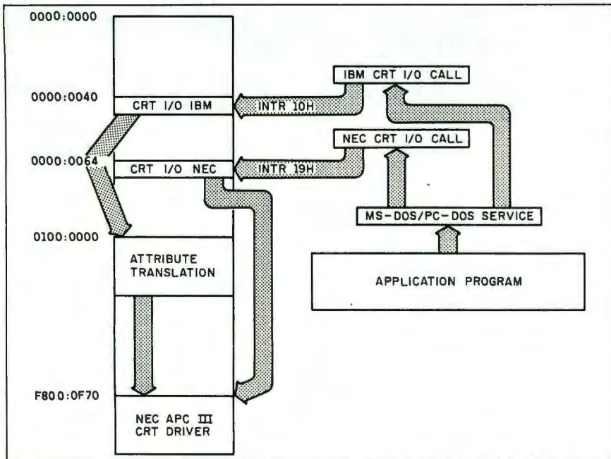
Figure 3: The program flow of the display I/O calls.
