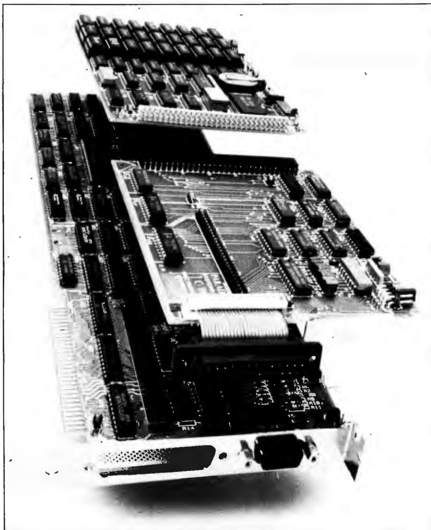
Photo 1: Modular Graphics Card from Paradise Systems fits into any full-size slot in an IBM PC or compatible. The connector at the bottom right of the photo mates with a cable from a monochrome TTL monitor. Also shown are two of Paradise's optional add-on modules: at the top is a combination RAM/clock card, and below that, a serial adapter card.
