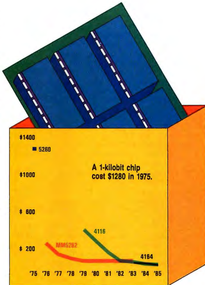
The cost of 64K bytes of RAM from 1975 to 1985, as found on the pages of BYTE magazines. Prices shown are for 512 of the 1-kilobit 5260 chip, 256 of the 2-kilobit MM5262 chip, 32 of the 2K-byte 4116 chip, and 8 of the 8K-byte 4164 chip.
