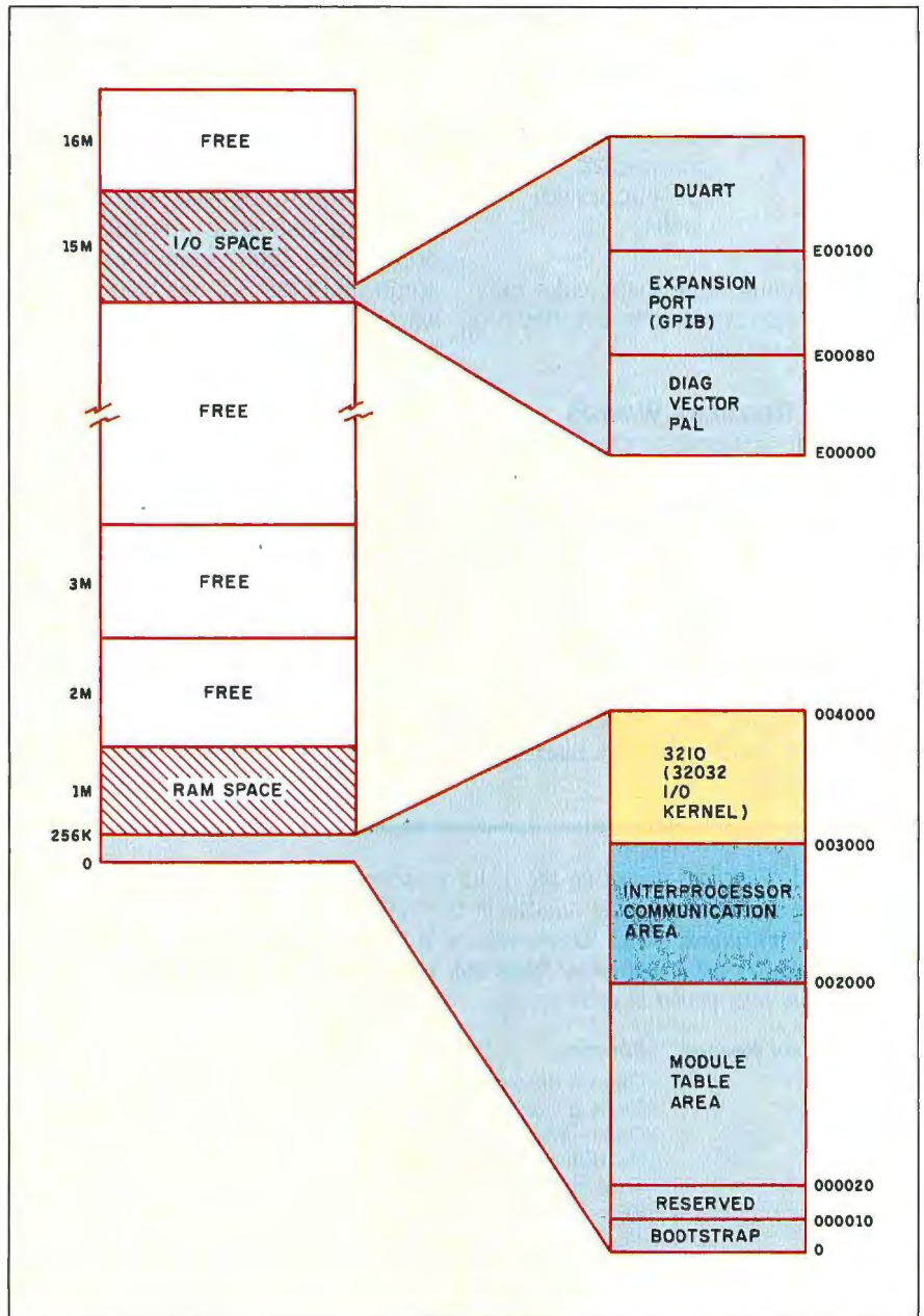
Figure 1: The DSI-32's memory map. 32IO is the I/O kernel that resides between locations 3000 and 4000. All addresses are in hexadecimal.
