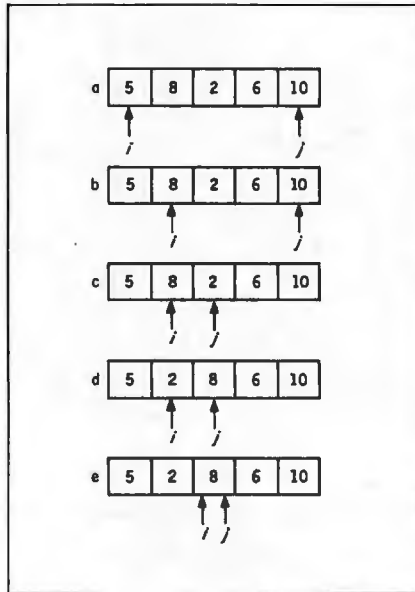
Figure 3: Partitioning of an array segment in Quicksort. In line a, i and j point to the beginning and end of the array, respectively. The pivot is taken to be the first element, here 5. In line b, i moves forward until the element it points to is greater than the pivot. In line c, j then moves down until it reaches an element less than or equal to the pivot. In line d, the two elements pointed to by i and j are swapped. And in line e, i then moves up again, becoming equal to j . This terminates the partitioning phase.
