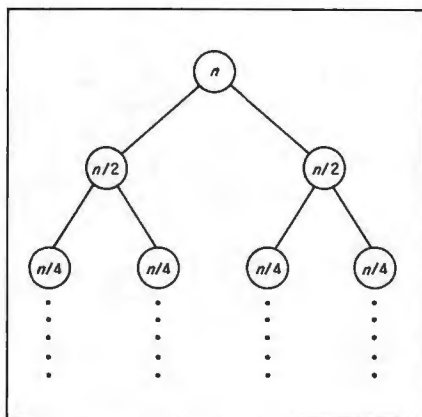
Figure 2: The Mergesort tree.
