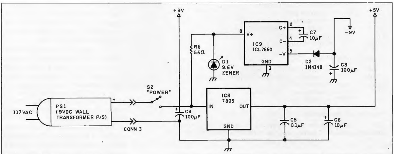
Figure 2: The power-supply adapter for the parallel-to-serial converter of figure 1.
