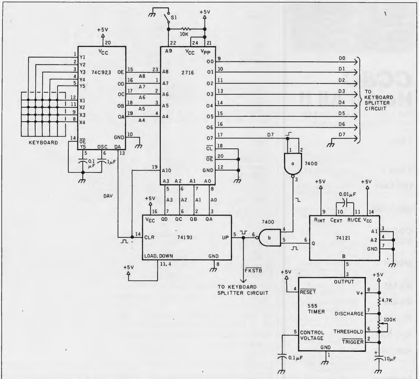
Figure 2: A schematic of the function-key-generator circuit.
