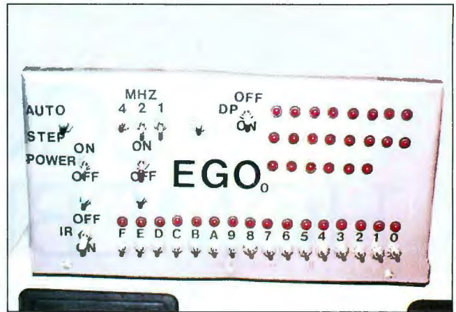
Photo 1: EGO, the author's homemade CPU, sits atop a Tandy 2000 that is used for uploading and downloading programs. The switch in the upper left corner allows the author to run EGO in single-step mode, and the row of LEDs along the bottom can be used to read either EGO's data bus or the CPU's instruction register.
