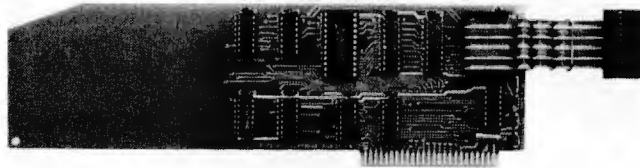
Writable ROM Board from Douglas Electronics.
