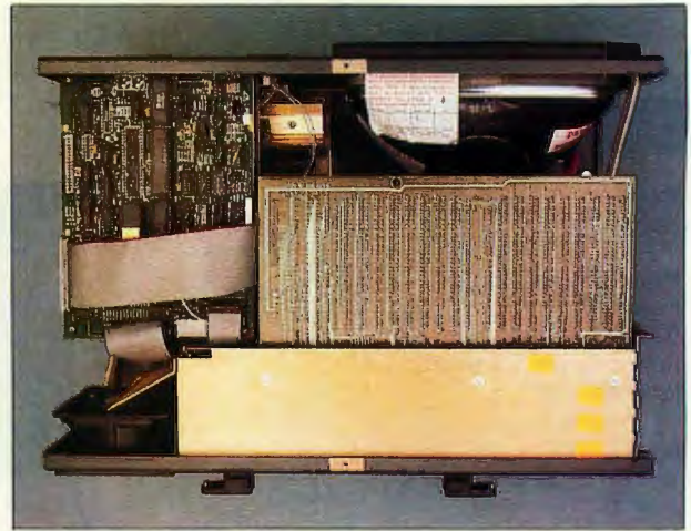
Removing the Kaypro 16 from its case reveals the expansion slot cage (bottom), the main memory board, and the hard-disk controller (left front).
