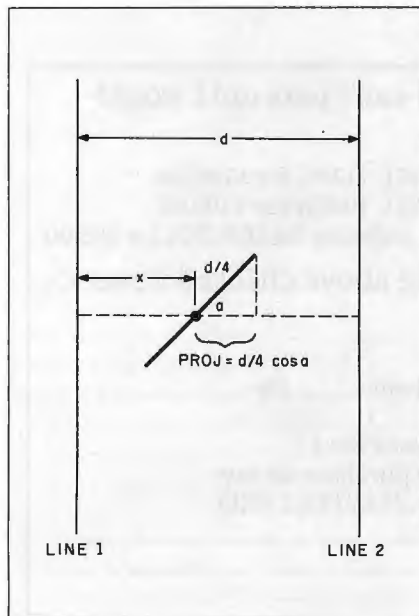
Figure 3: The geometry of the Buffon needle experiment.
