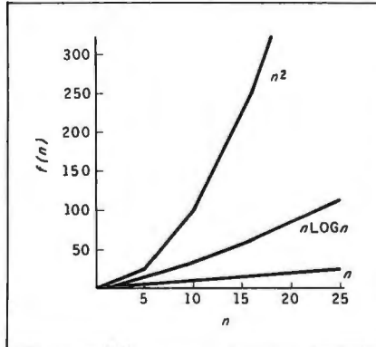
Figure 1: Rates of growth of some common functions.
