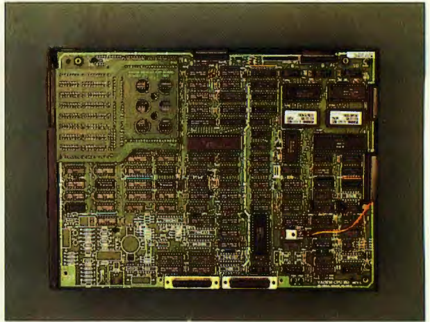
Inside the Osborne 3. Parallel and serial connectors are at the bottom.
