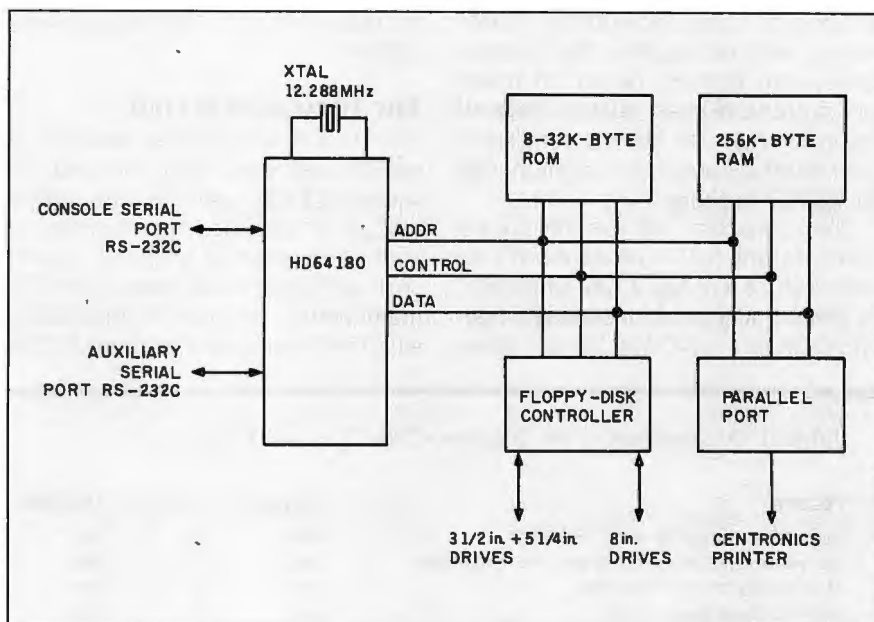
Figure 1: Block diagram of the SB180 single-board computer.
