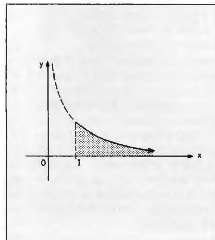
Figure 2a: Graph of y = \frac{1}{x} on [1, \infty) .
