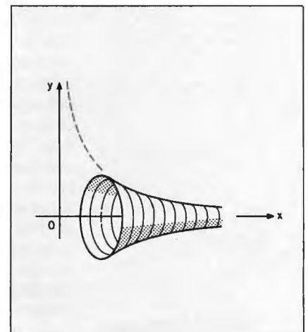
Figure 2b: The funnel formed by revolving 2a around the x-axis.
