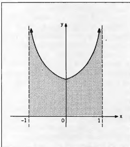
Figure 1: Area under y = \frac{1}{\sqrt{1-x^2}} .
