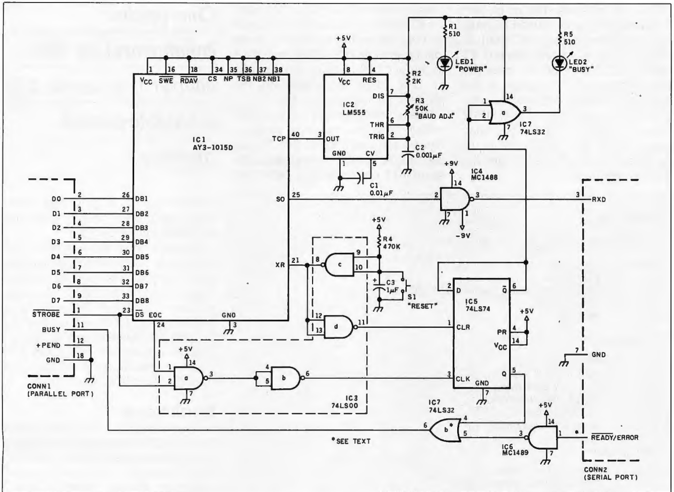
Figure 1: A schematic for the parallel-to-serial adapter. The UART (IC1) converts the 8 bits coming in at the parallel port
