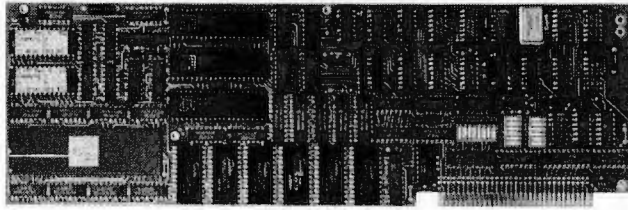
PC FFT coprocessor card from Ariel.
