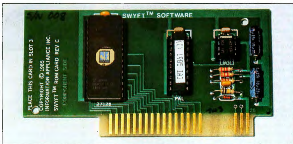
The SwyftCard add-in for Apple IIe computers.
