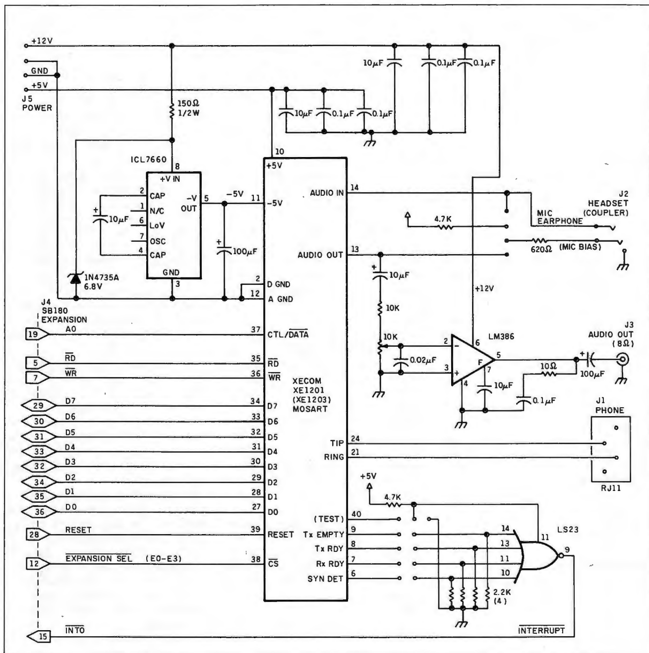
Figure 1: The schematic diagram of the Circuit Cellar COMM180 modem expansion board.
