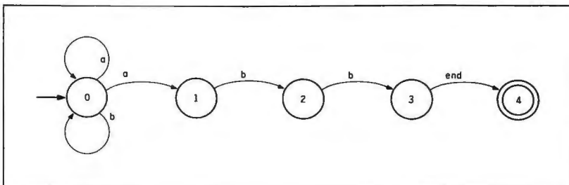
Figure C: This network involves relaxing the rule that requires a unique set of transition values on each arc. Since there are two "a" transitions, the network follows both.
