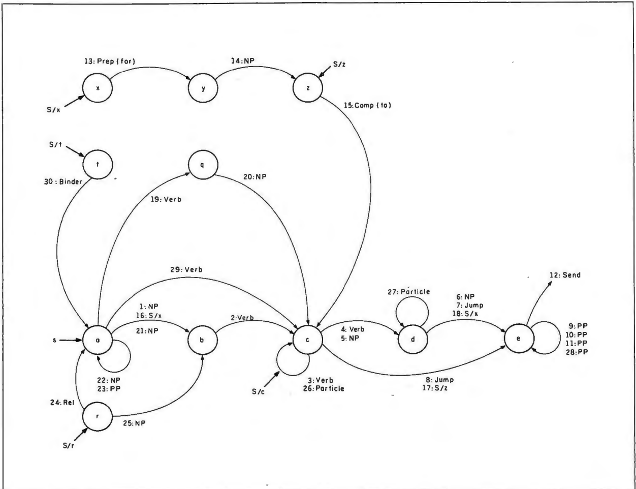
Figure H: The S/ (sentence) network.
