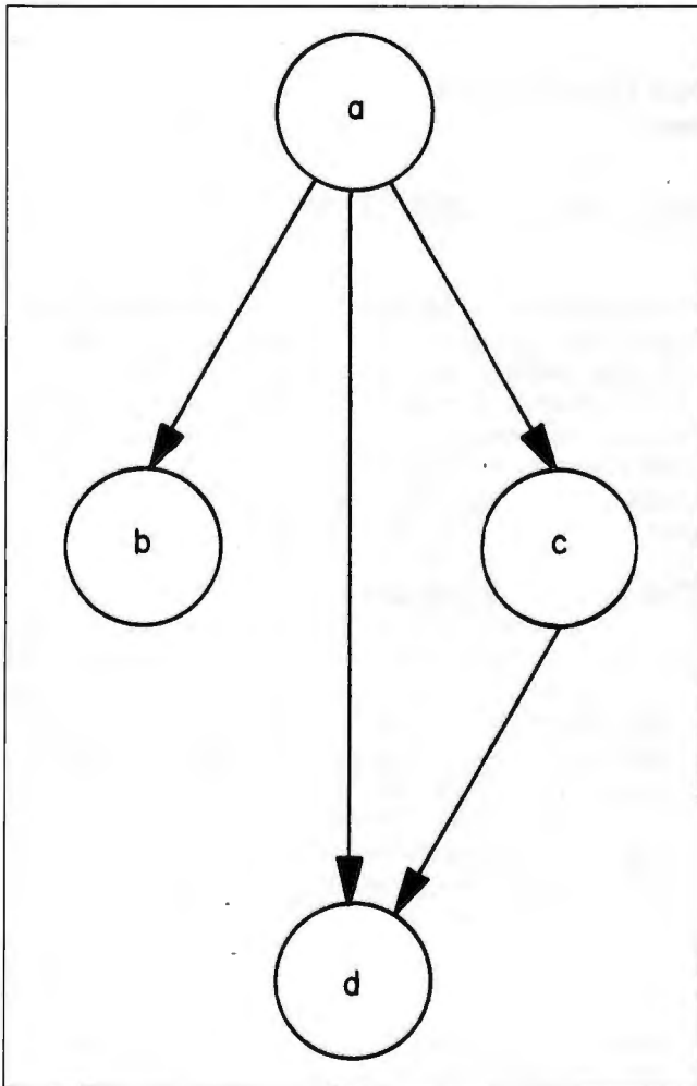
Figure 1: A context graph for a conversation in which message a was the initial message of the conversation. Messages b and c were submitted after their respective authors had read message a , but independently of each other. Message d was submitted after its author had viewed messages a and c but before he had viewed message b .
