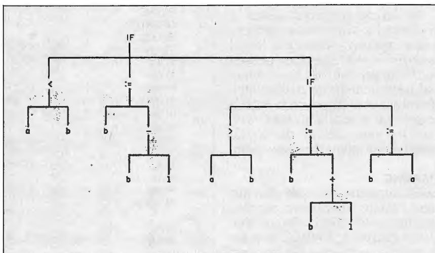
Figure 2: Parse tree for the SIMPL statement IF a < b THEN b := b - 1; ELSIF a > b THEN b := b + 1; ELSE b := a.
