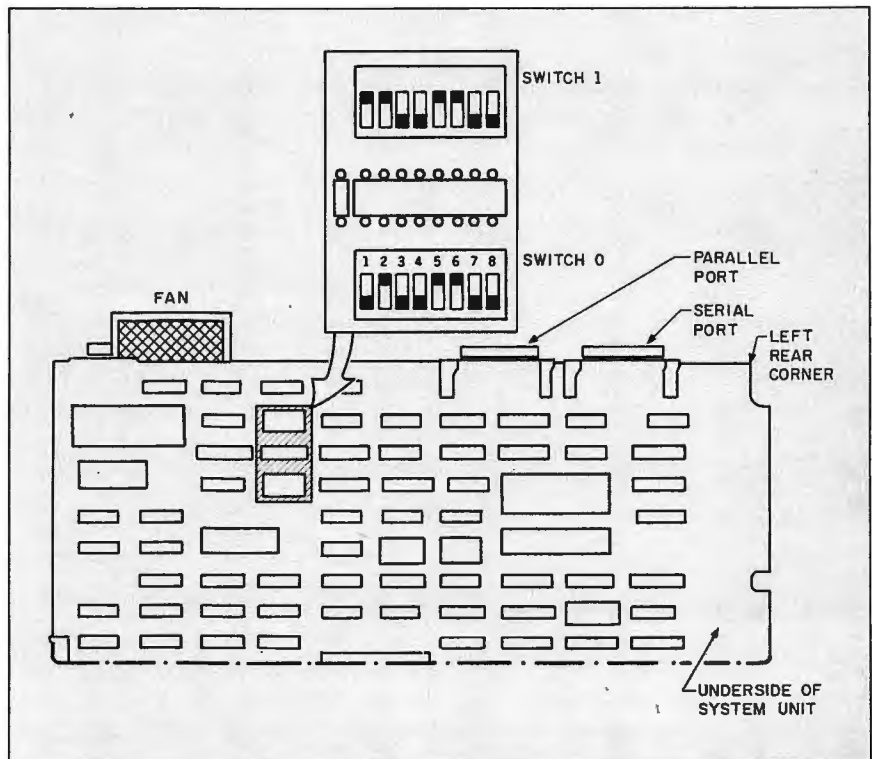
Figure 1: The bottom right corner of the AT&T PC 6300's motherboard, showing the location of DIP switches and switch settings for 640K bytes of RAM.
