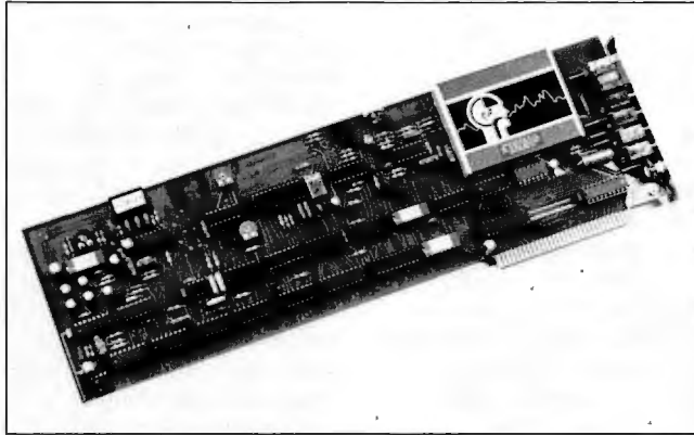
The CompuFone board from Computalkers Consultants.
