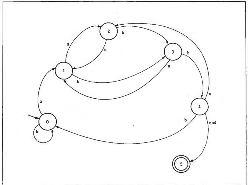
Figure D: This network performs the same function as the one in figure C. However, it is much more complex because it has a unique transition value on each arc and follows only one path.
