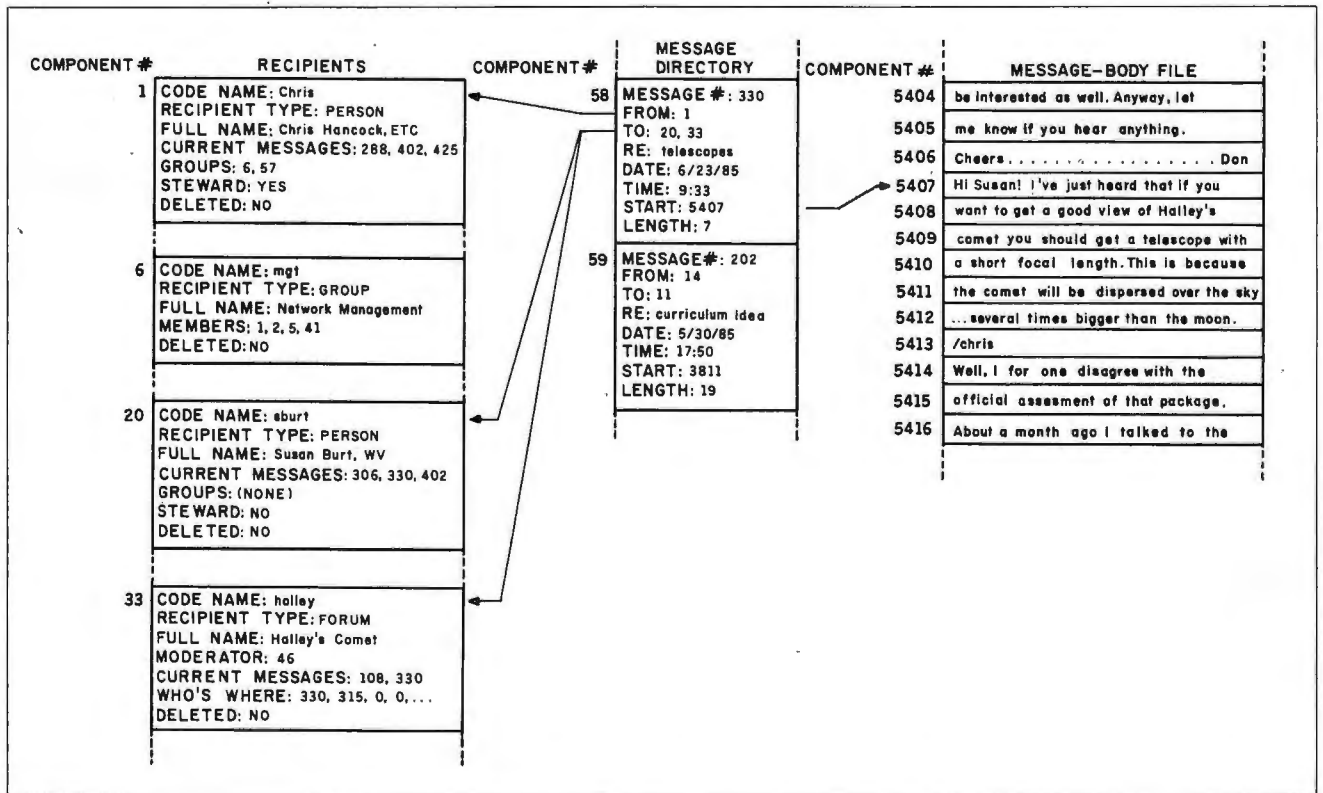
Figure 2: An example of Common Ground's three data files, showing how the different components are linked to one another. The WHO'S WHERE entry in the halley forum is a list showing how far recipients have read. For example, the 330 in the first position indicates that recipient 1 has read up to message 330. The 315 in the second position indicates that recipient 2 has read up to message 315.
