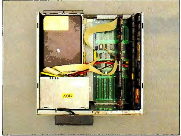
The inside of the AT&T PC 6300 showing disk drive, power supply, and motherboard with expansion connectors.
