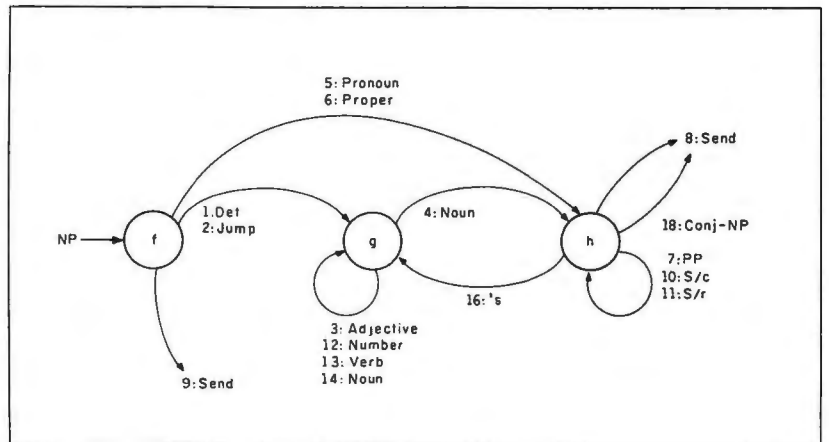
Figure G: The NP (noun phrase) network.
