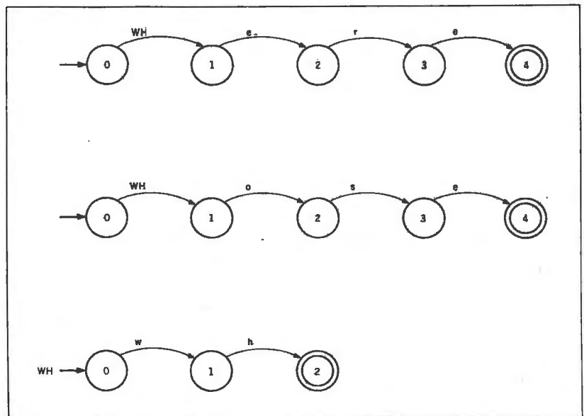
Figure E: The WH network replaces two arcs and states and matches "wh."
