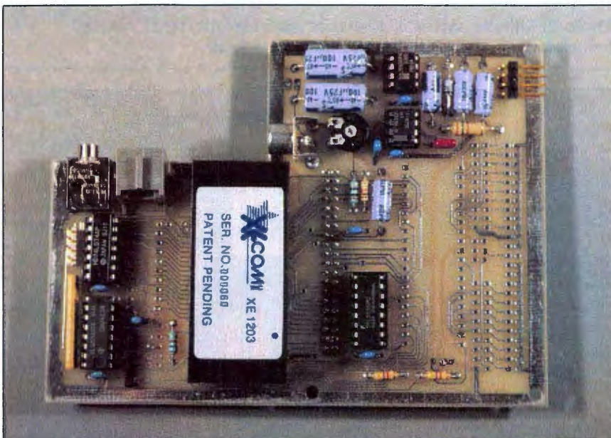
Photo 1: A prototype of the COMM180 expansion board, shown here populated with the MOSART communications chip and its supporting circuitry.
