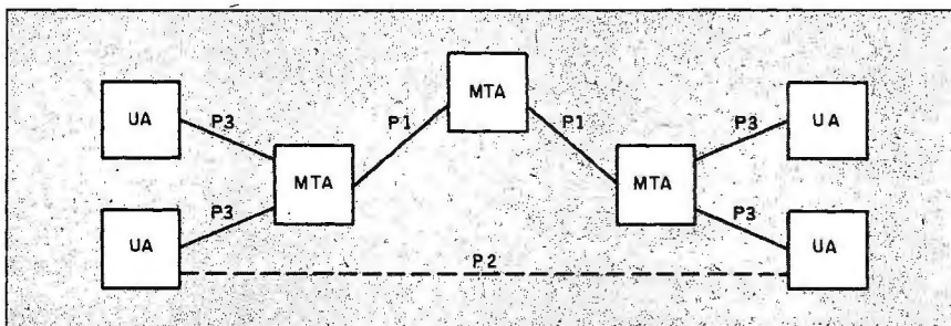
Figure 5: This figure shows how messages are passed from UAs (user agents) via one or more MTAs (message transfer agents) to the recipient UA in the MHS model. The P1 protocol is used between MTAs, and the P3 protocol is used between a UA and an MTA. The messages passed via P1 and P2 are formatted according to the P2 protocol, but this information is not interpreted by the MTAs, so the P2 protocol can be seen as a protocol between UAs.
