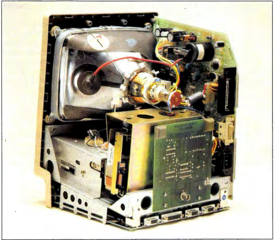
Photo 2: An interior shot of a HyperDrive-equipped Mac. The hard disk is the vertically mounted box. The circuit board in front of the hard disk is not part of the HyperDrive; it is an enhancement that gives the Mac an external video output jack.
