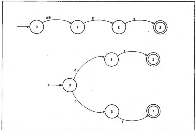
Figure F: The X subnetwork replaces arcs and states matching either "er" or "os."
