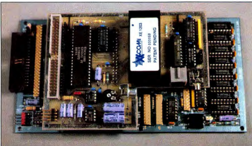
Photo 3: The COMM180 modem/SCSI board rides piggyback on the SB180 single-board computer, connecting via the SB180's expansion I/O connector.
