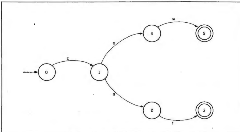
Figure B: A simple network that recognizes either "cat" or "cow."
