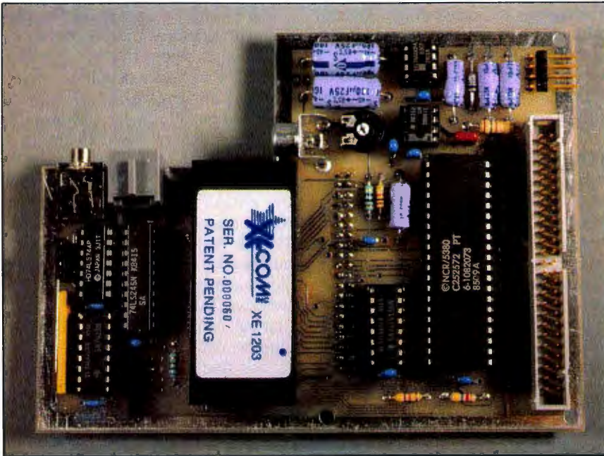
Photo 2: With the addition of a few chips and a connector, the COMM180 from photo 1 can also support an SCSI hard-disk interface.
