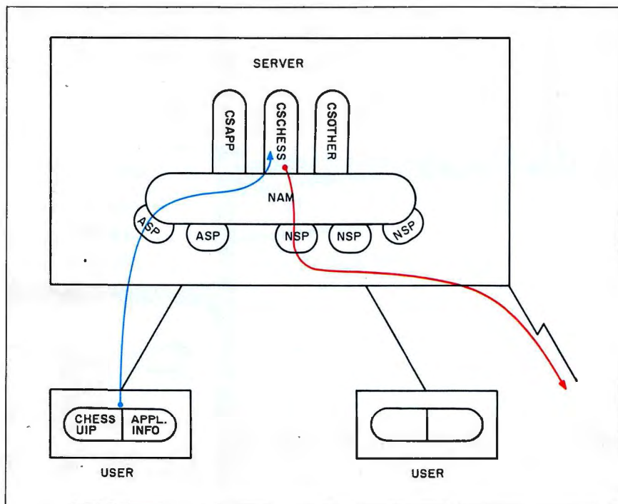
Figure 2: GRANDiose server internal organization. The NAM routes commands to the CSPs that contain the application-specific code. The ASPs and NSPs transmit and receive information to and from the server. The UIP exists within the user's sphere; half of the UIP communicates with the server, and the other half interprets the application-specific information. The blue line from one user represents the transmission of a chess move from the CHESS UIP through an ASP to the NAM and on to the CSCHES application. CSCHES then forwards the move, via the red line, through an NSP out over the network.
