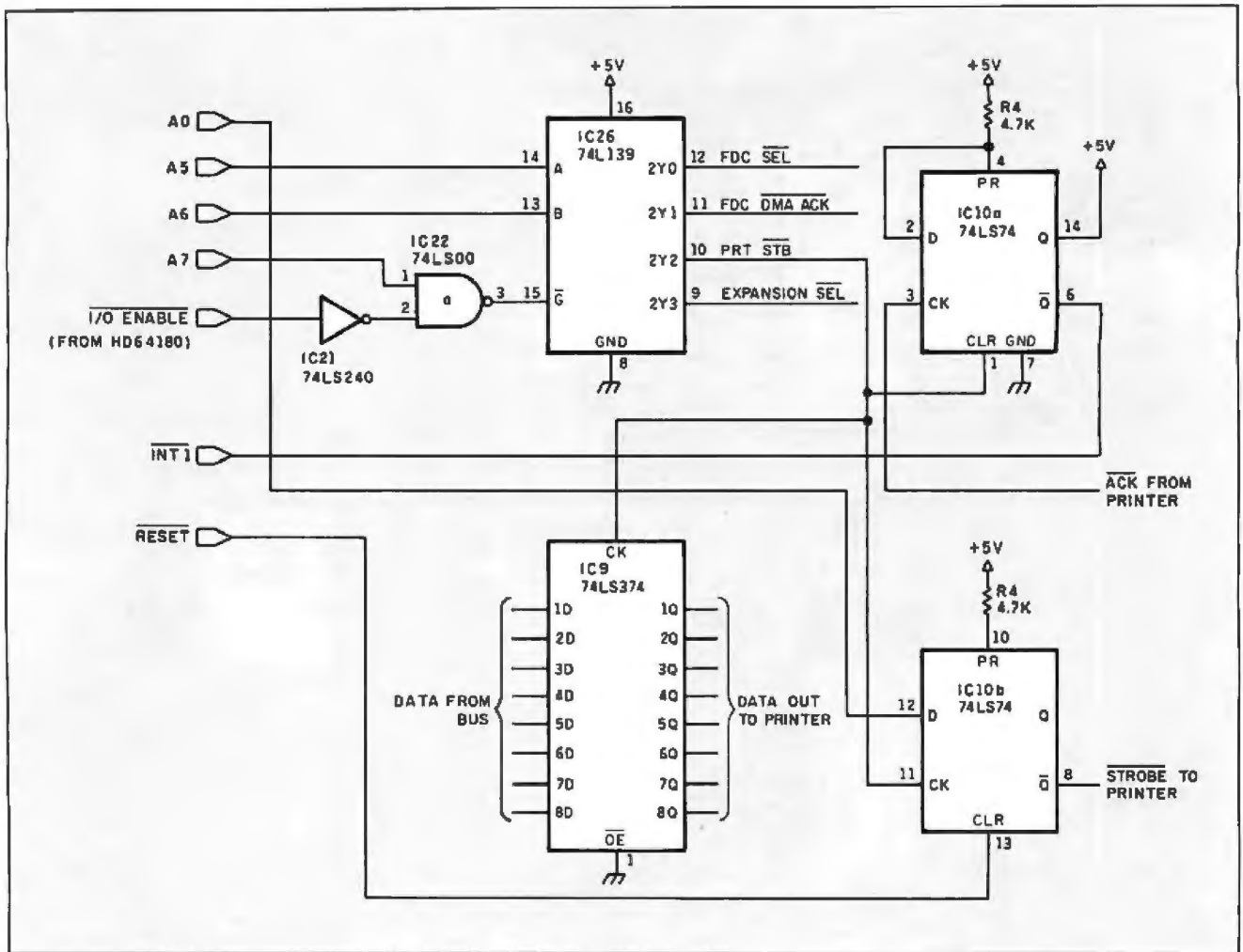
Figure 5: The SBI80 printer port.
