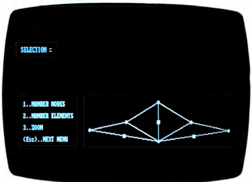
Photo 4: The same truss plotted with 10,000-pound loads and an exaggeration ratio of 30. Rectangles have been placed by the program through members that exceed the design stress.
