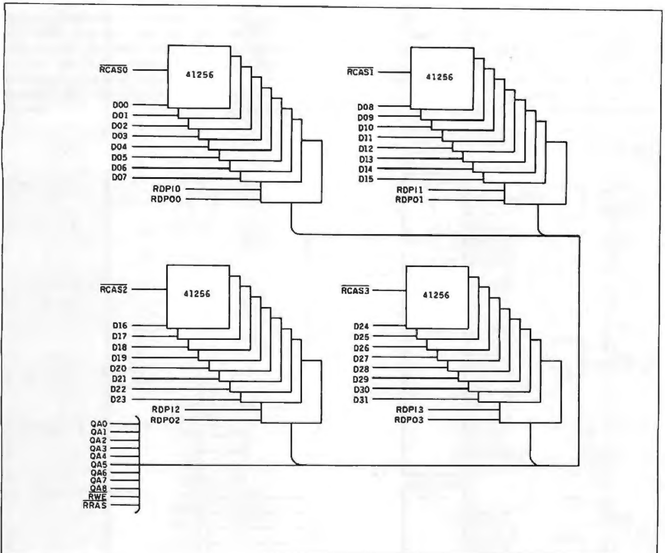
Figure 6: Memory array.
