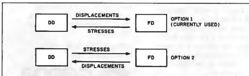
Figure 9: Coupling options for the hybrid DD/FD model.
