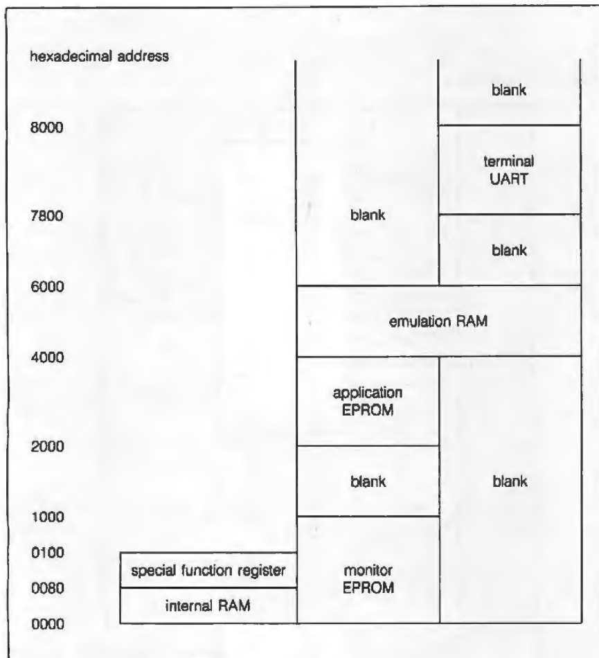
Figure 2: The emulator board's memory map.
