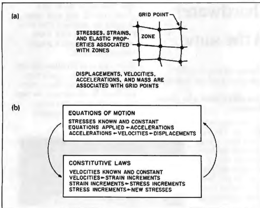
Figure 8: Details of the FD method; (a) shows a portion of a typical FD mesh consisting of arbitrary zones with a grid point at each corner; (b) illustrates the FD calculation sequence.
