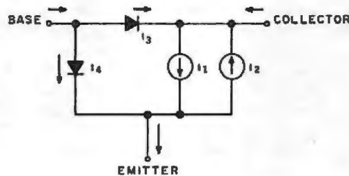
Nonlinear Hybrid- \pi Model with Early Voltage Effect
