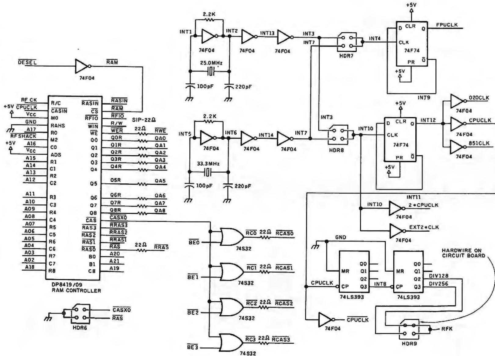
Figure 5: RAM controller circuitry.
