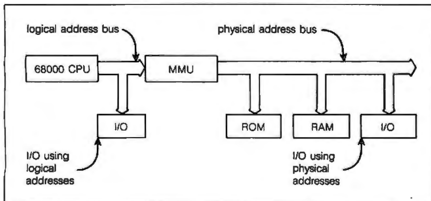
Figure 8: Address translation.
