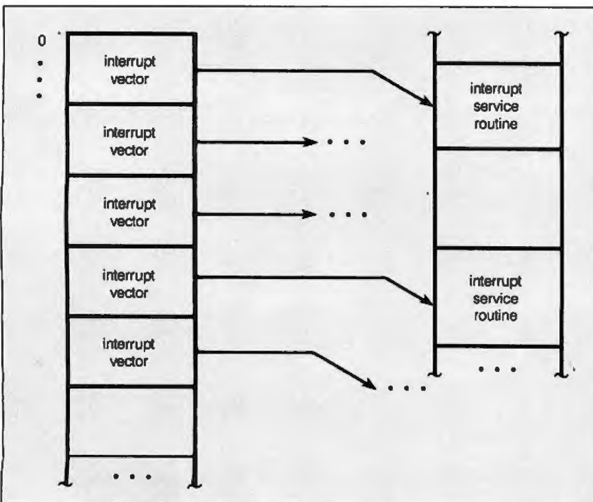
Figure 7: Vectored interrupts.
