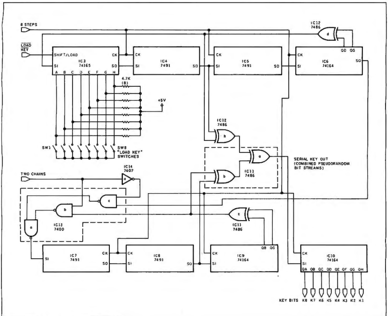
Figure 3: Key-generator logic.
